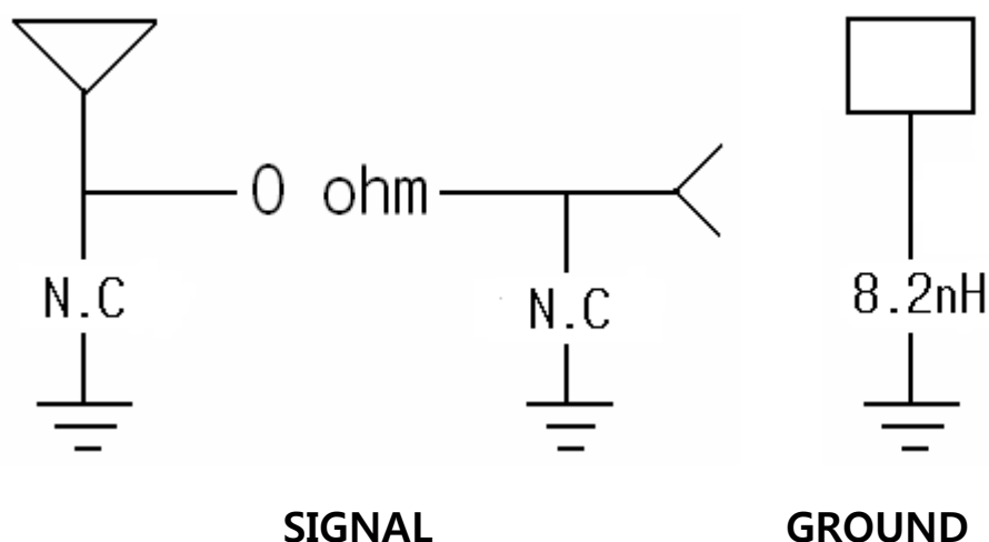
<Figure 2.3.1 Matching circuit>
