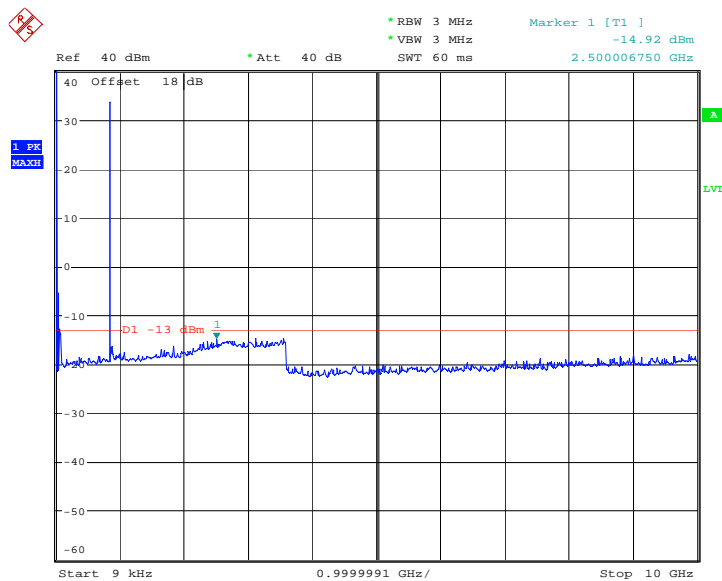
(Plot A4.:GSM 850MHz Channel = 128, 9KHz to 10GHz)
