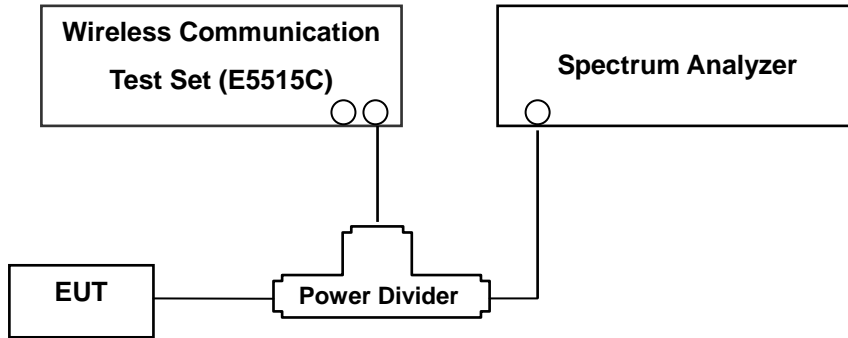
(Configuration of conducted Emission measurement) Test Procedure
