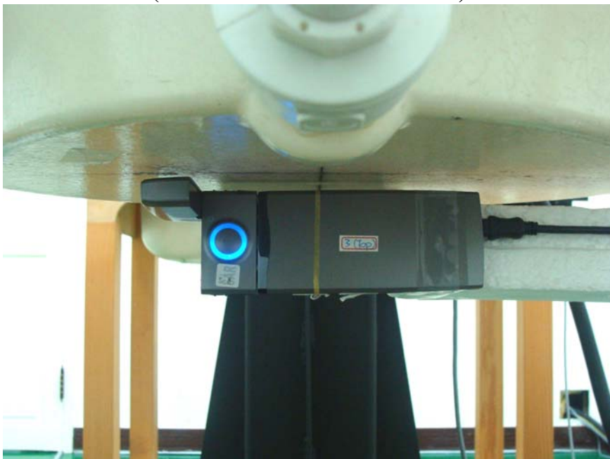
DUT Left Side with Phantom 0.5cm Gap (Antenna in Vertical Position)
