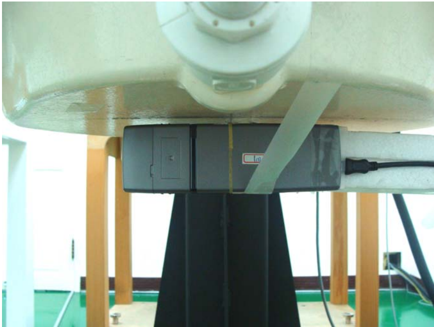
DUT Right Side with Phantom 0.5cm Gap (Antenna in Horizontal Position)
