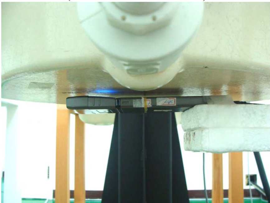
DUT Face with Phantom 0.5cm Gap (Antenna in Horizontal Position)
