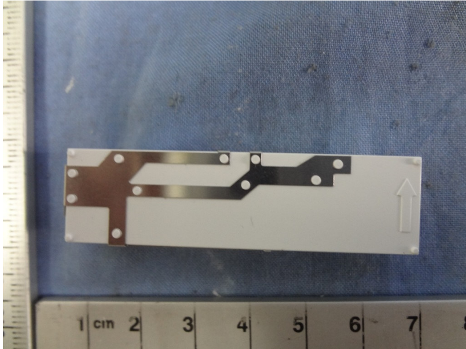
CDMA Antenna
