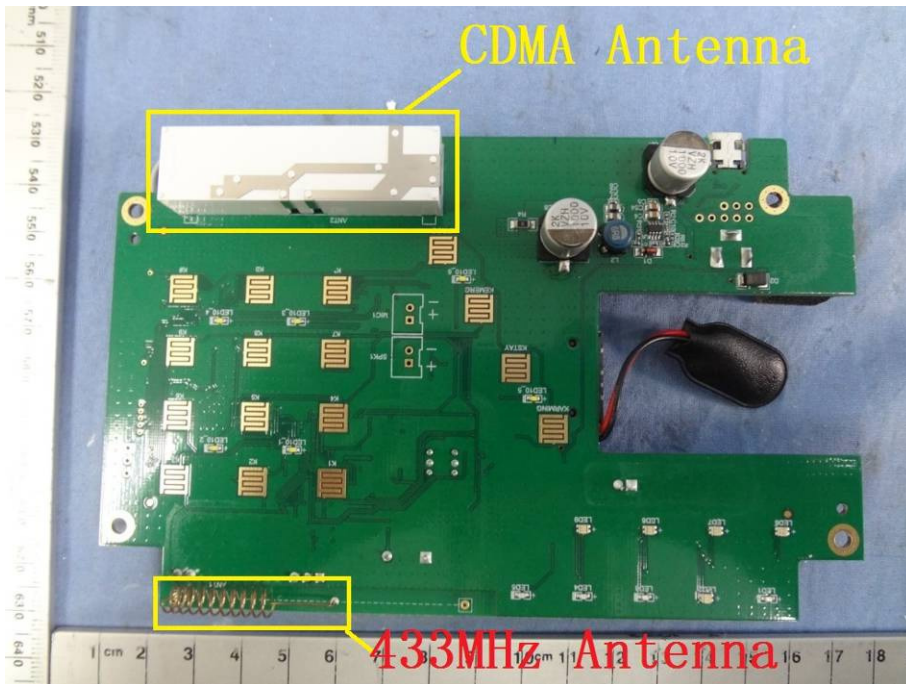
433MHz Antenna
