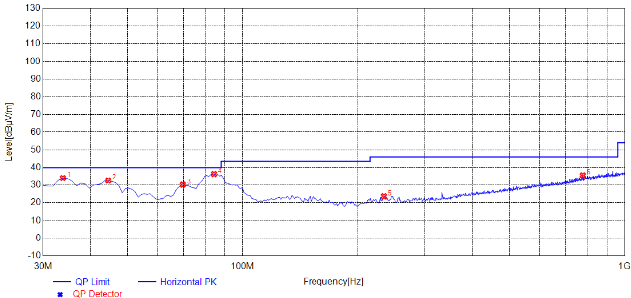
Radiated Emission Test –Horizontal -3m Below 1G
