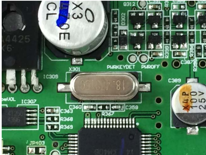
Oscillator view 3
