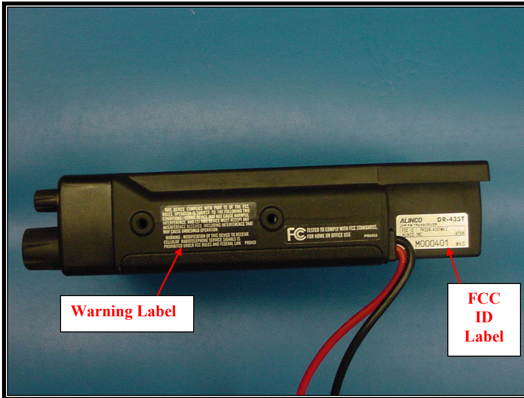
PHOTOGRAPH 3: FCC ID LABEL AND WARNING LABEL LOCATIONS ON RIGHT SIDE OF EUT
