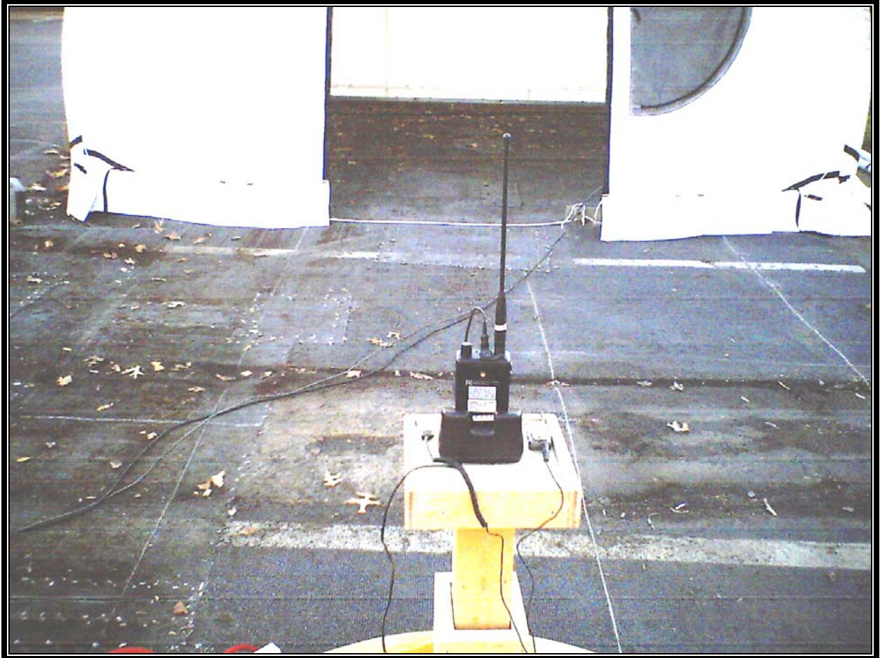
Photograph 4: Radiated Emissions Test Configuration (Rear View)
