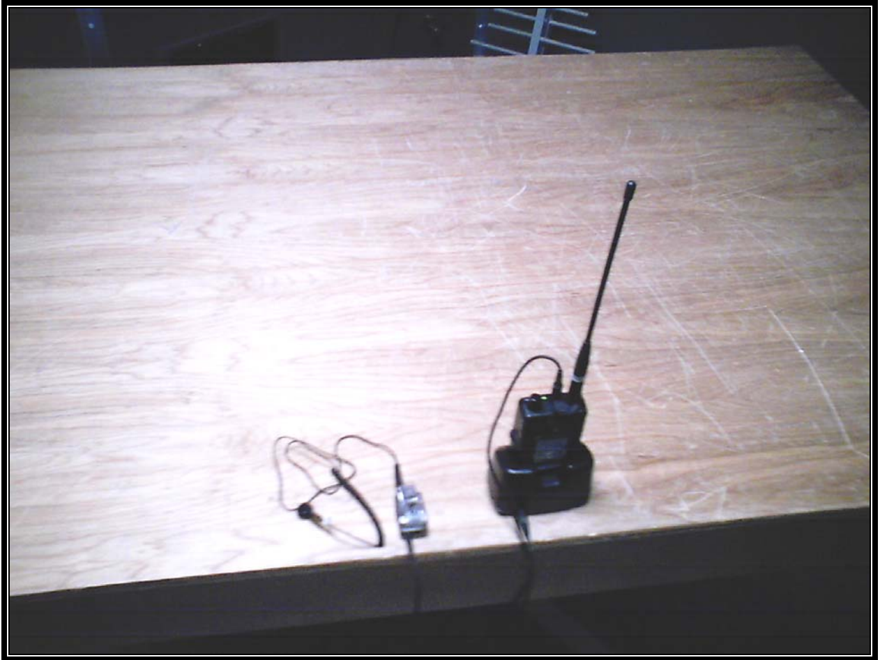
Photograph 6: Conducted AC Emissions Test Configuration (Rear View)
