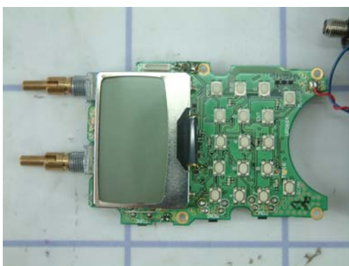
PCB 1 solder
