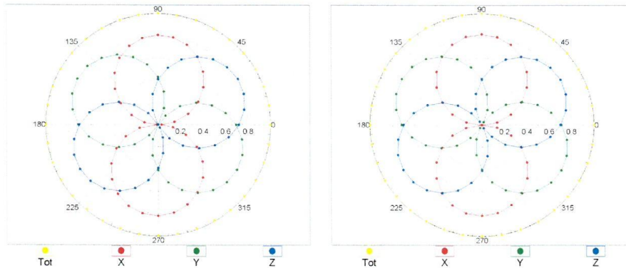
f=600 MHz,TEM
