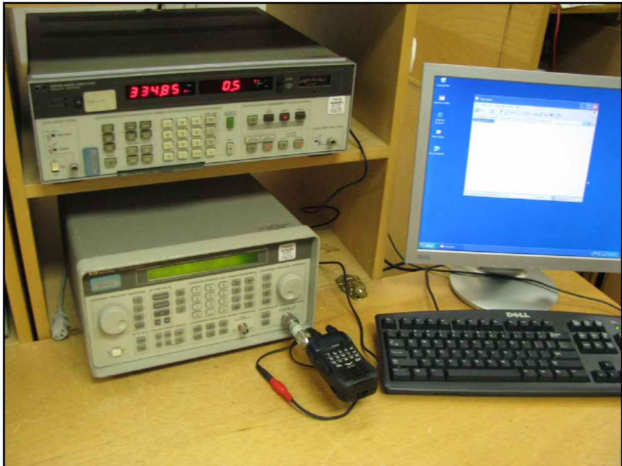
Photograph 4: 38 dB Rejection Test Configuration
