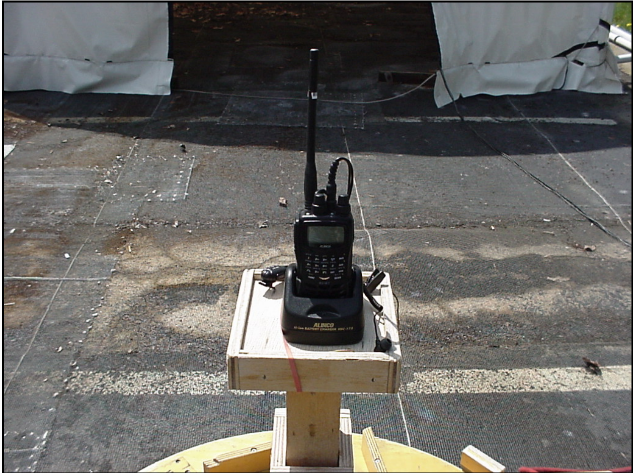
Photograph 2: Radiated Emissions Test Configuration (Front View)
