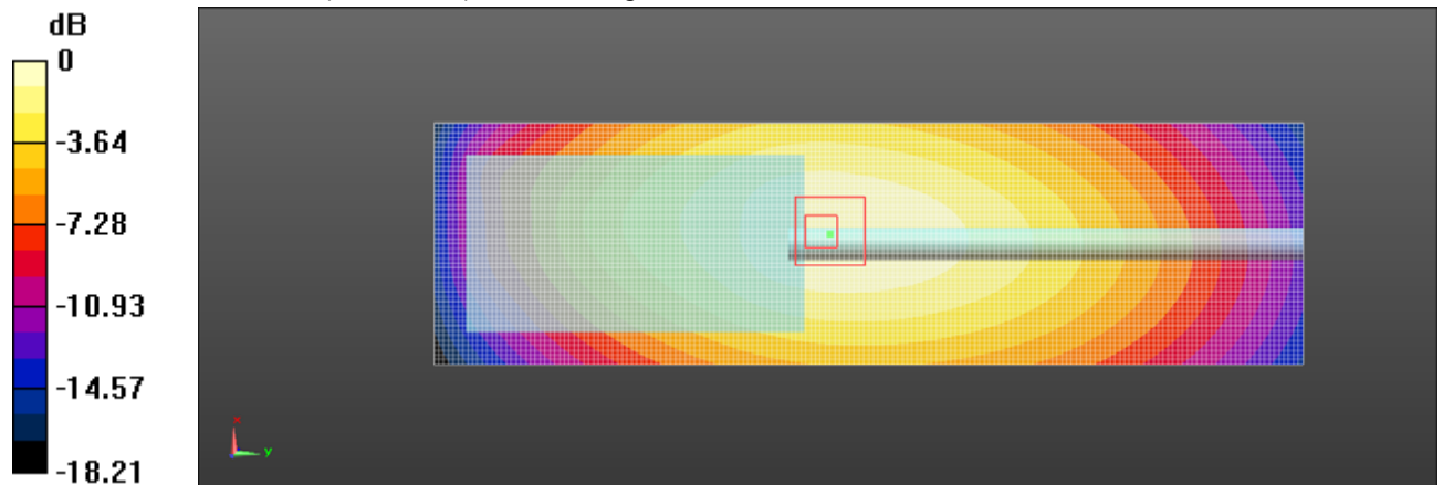
Plot 5: Body-worn for Digital Modulation at 12.5KHz Channel Separation With A1, B1,BC1,S1and C1; Front towards Ground 450.50 MHz
