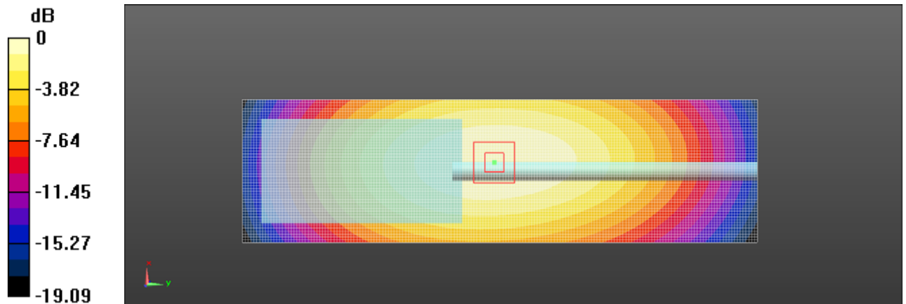
Plot 3: Body-worn for Digital Modulation at 12.5KHz Channel Separation With A1, B1,BC1,S1and C1; Front towards Ground 422.50 MHz
