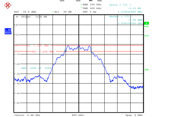
BLE_2M_High_Channel
