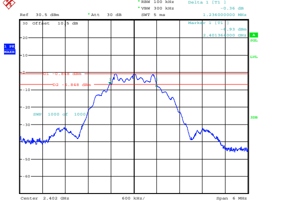
BLE_2M_Low_Channel
