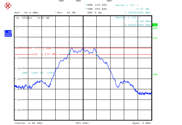
BLE_2M_Middle_Channel
