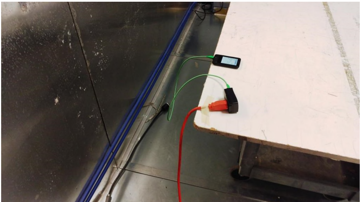
Figure 8: Equipment Under Test – AC Conducted Emissions
