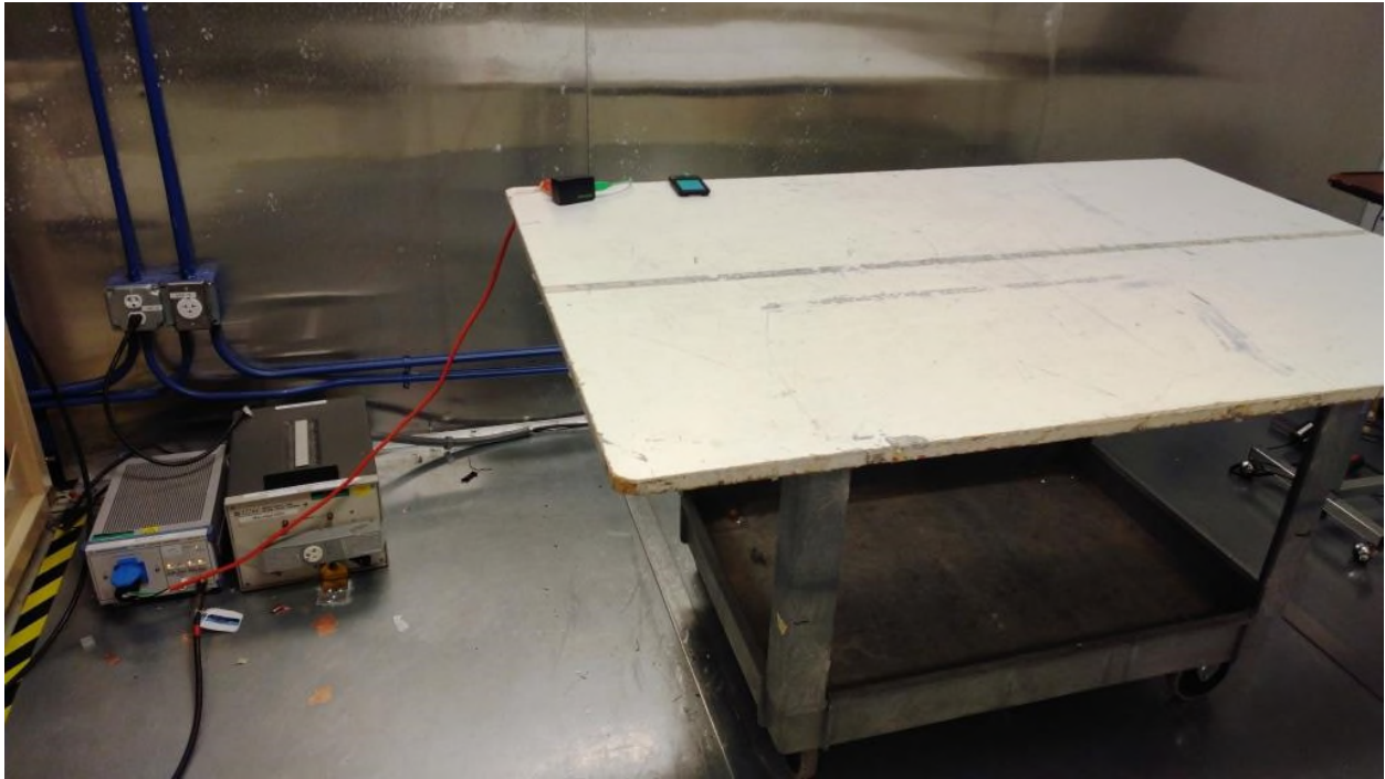
Figure 7: Equipment Under Test – AC Conducted Emissions
