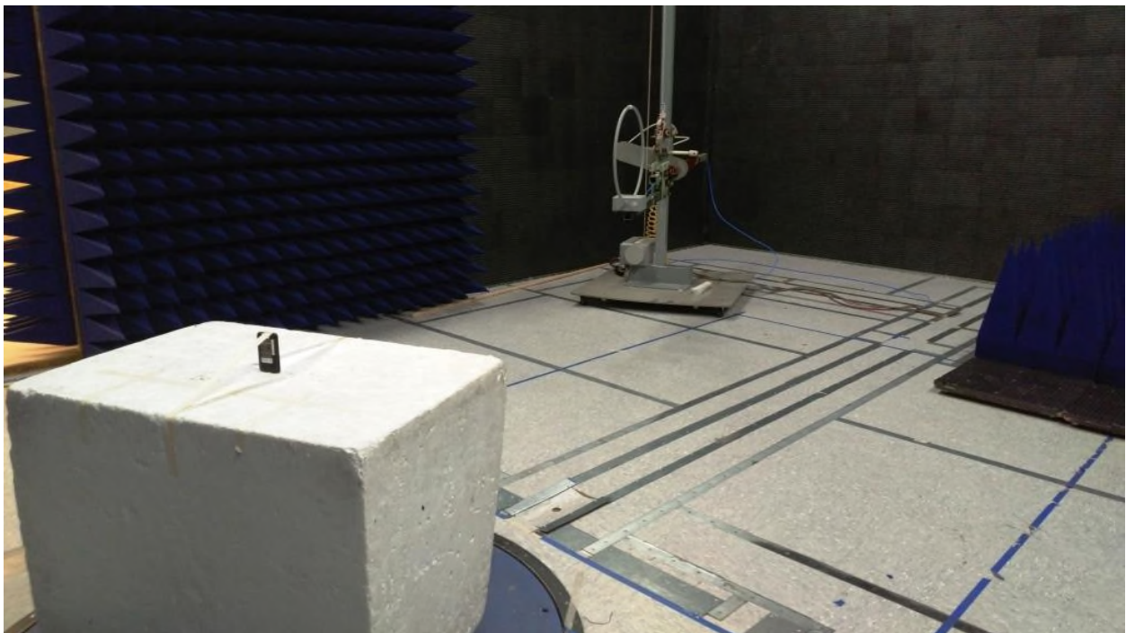
Figure 2: Equipment Under Test – Radiated Emissions – 9kHz-30MHz
