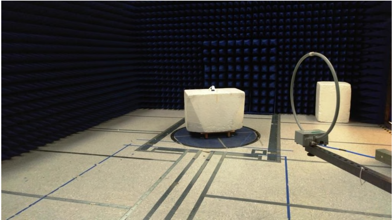
Figure 1: Equipment Under Test – Radiated Emissions – 9kHz-30MHz
