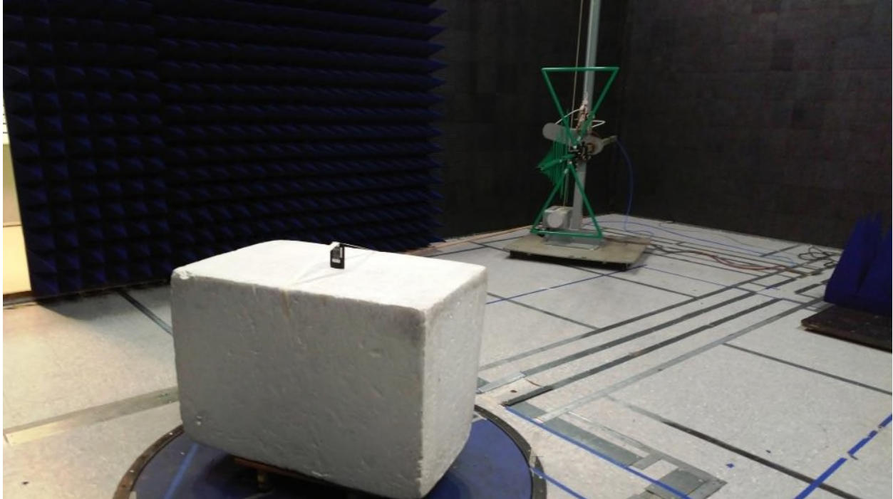
Figure 4: Equipment Under Test – Radiated Emissions – 30-1000MHz
