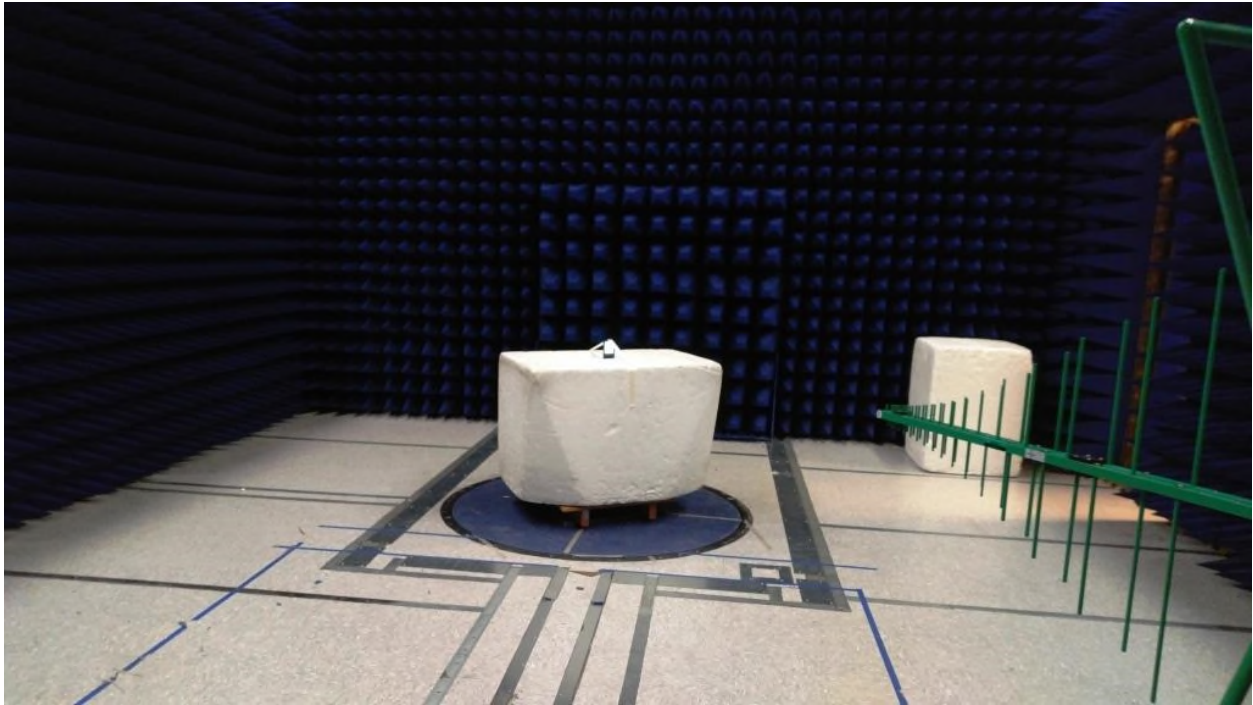
Figure 3: Equipment Under Test – Radiated Emissions – 30-1000MHz
