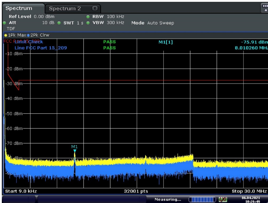
BLE High Channel (9kHz to 30MHz)
