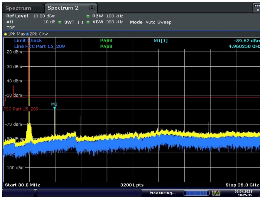
BLE High Channel (30MHz to 25GHz)
