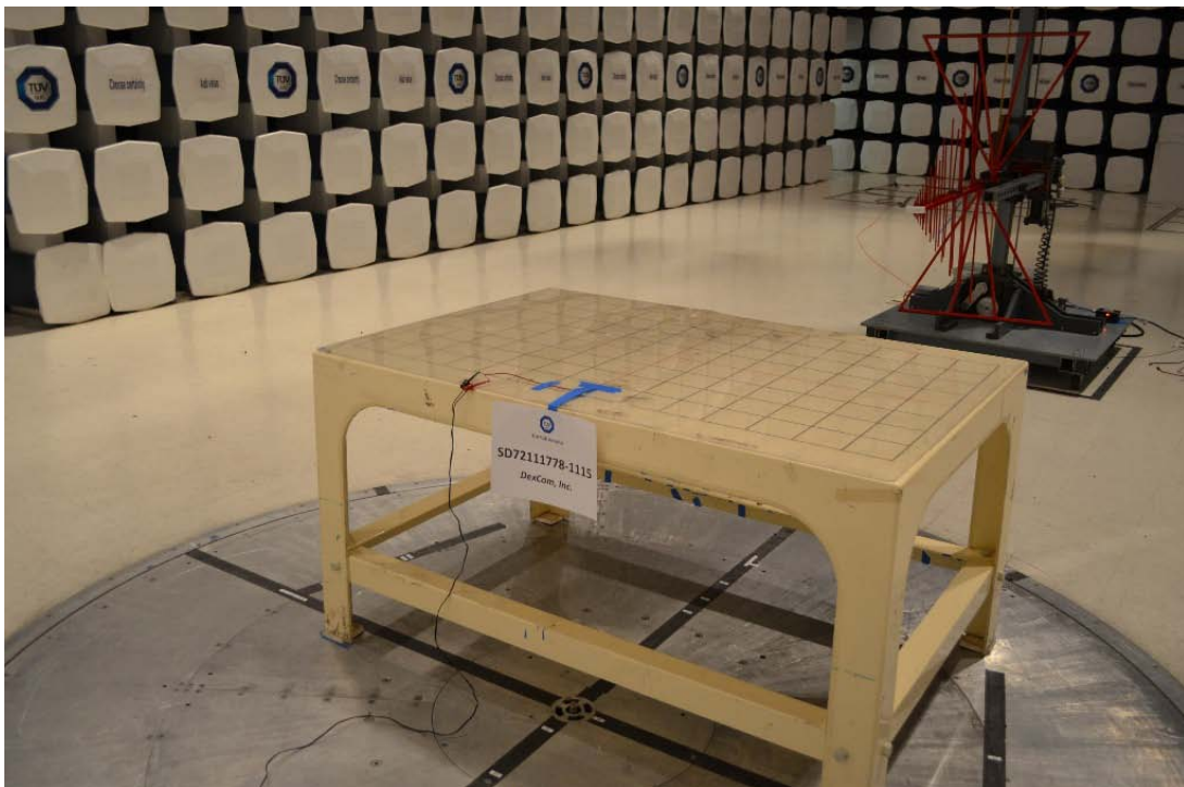
Radiated Emissions
