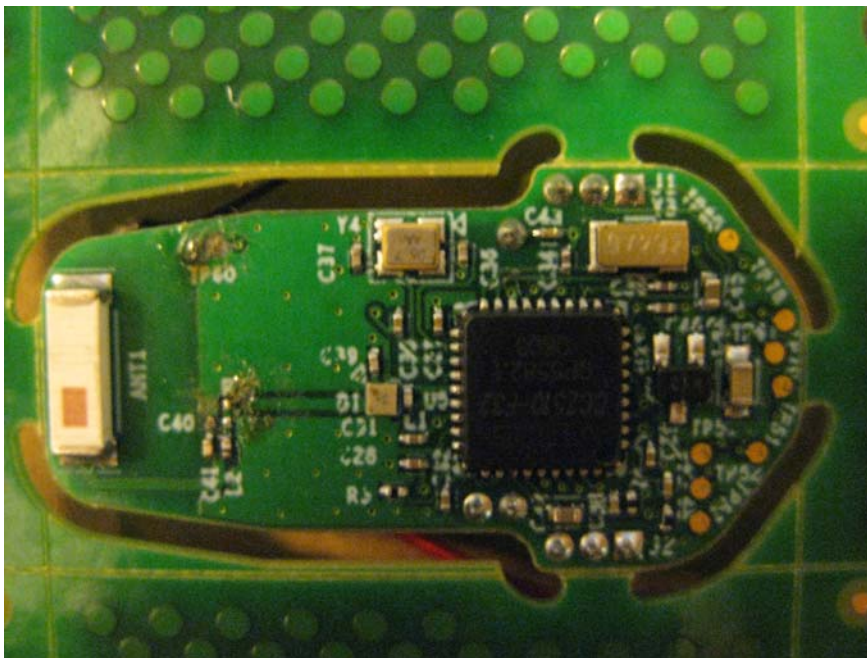
Back side of transmitter open for inspection
