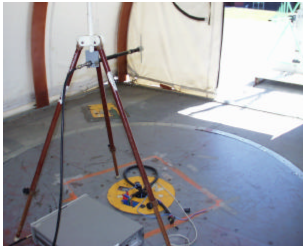
Substitution Method
