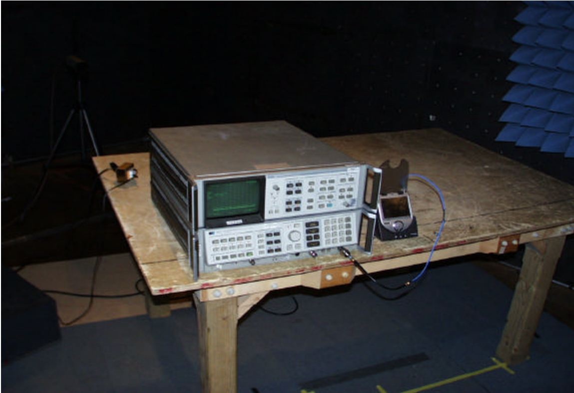
FREQUENCY/VOLTAGE SETUP
