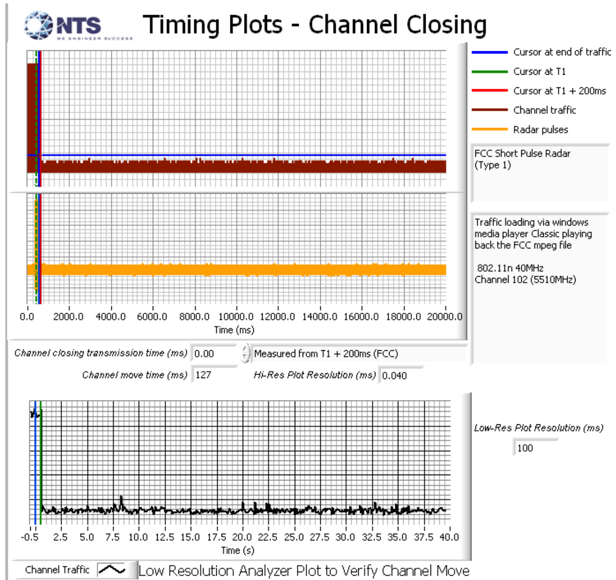
Figure 4 Channel Closing Time and Channel Move Time (40MHz mode) – 40 second plot
