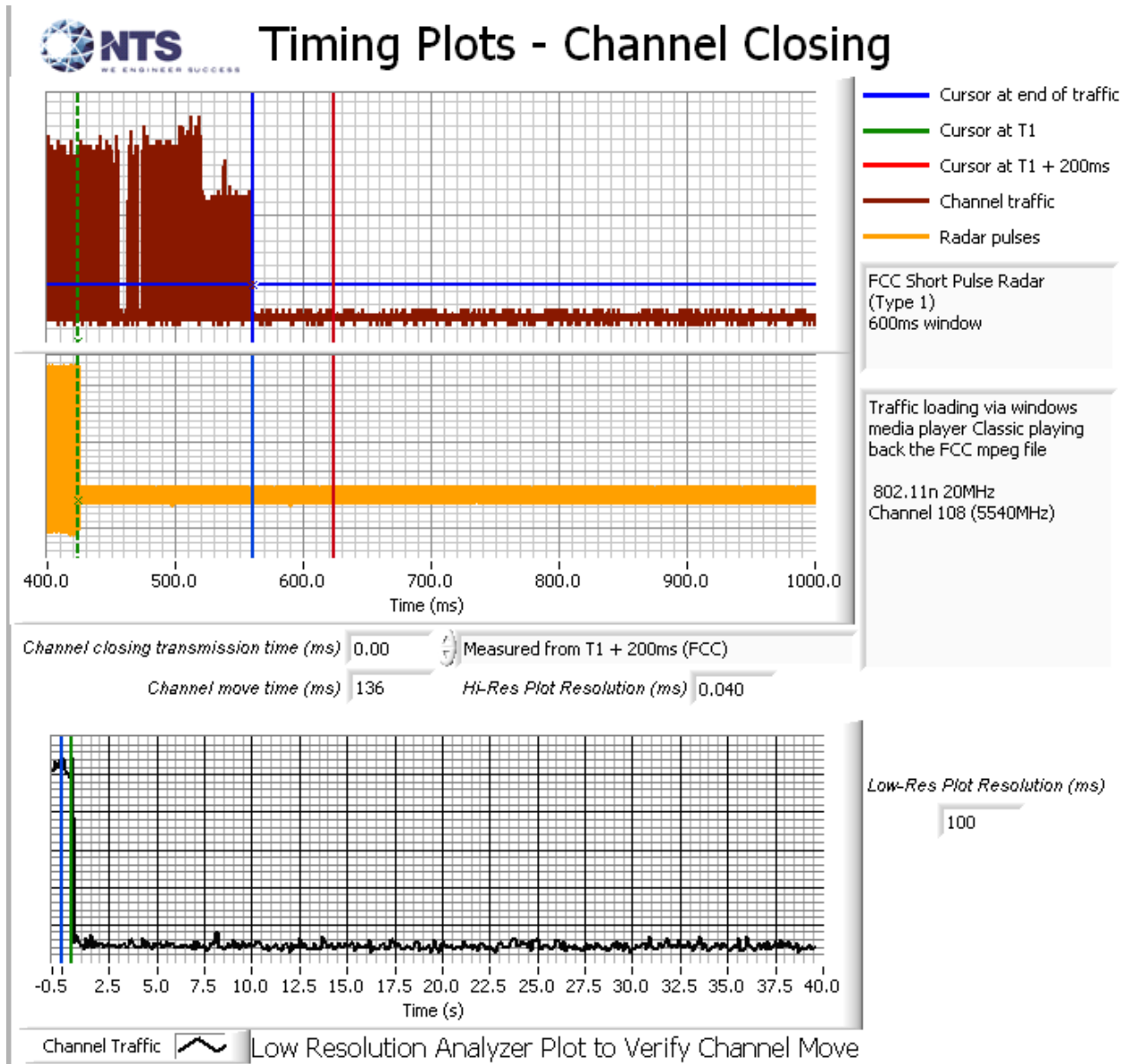
Figure 3 Close-Up of Transmissions Occurring More Than 200ms After The End of Radar (20MHz mode)
