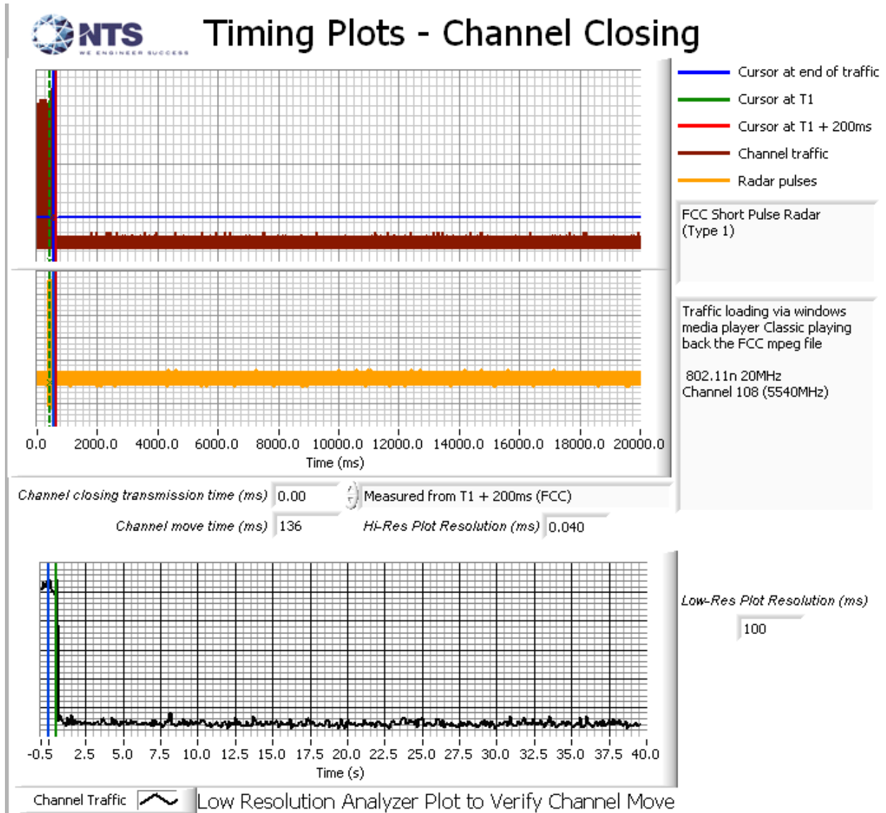
Figure 2 Channel Closing Time and Channel Move Time (20 MHz mode) – 40 second plot
