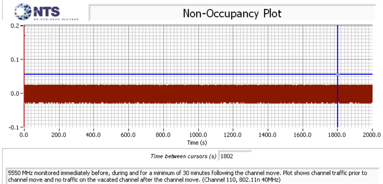
Figure 6 Radar Channel Non-Occupancy Plot (mode)
