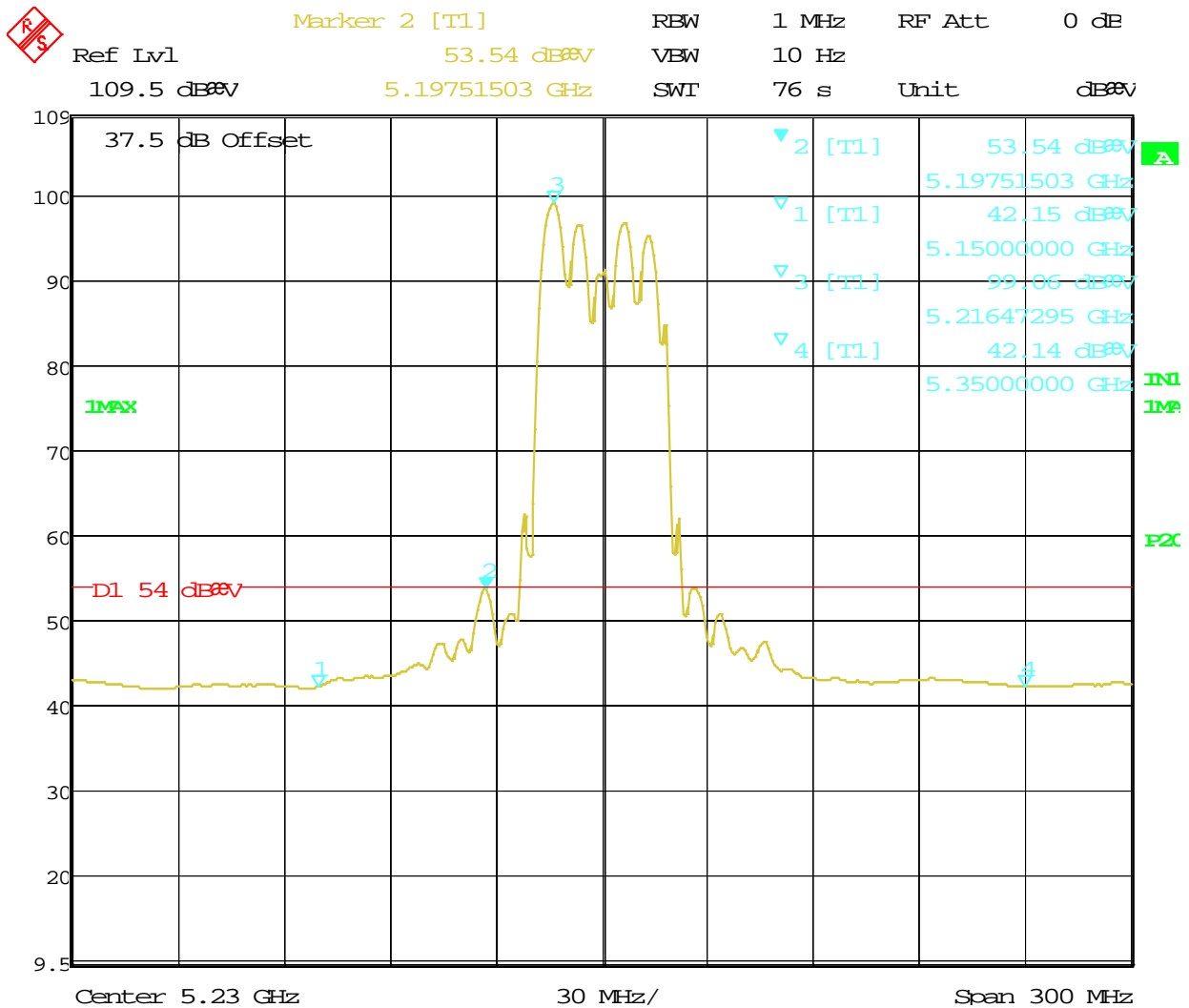
Figure 99: Radiated Emission at the Edge for Channel 5230 MHz at 13.5Mbps – Vert (Ave.)
