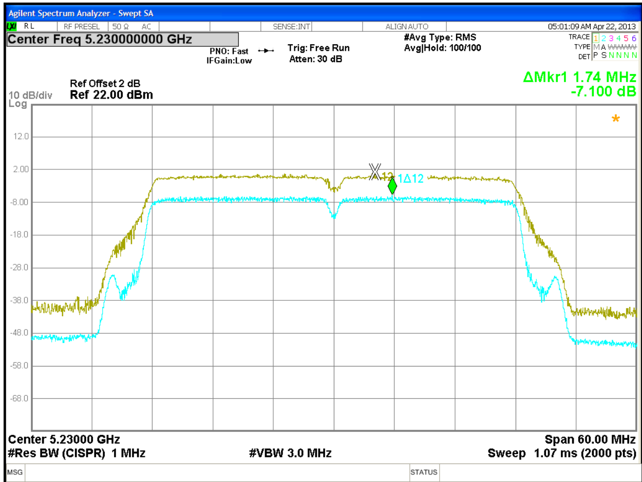
Figure 58: Peak Excursion, 5230 MHz at 802.11n, Chain 1 – 13.5 Mbps
