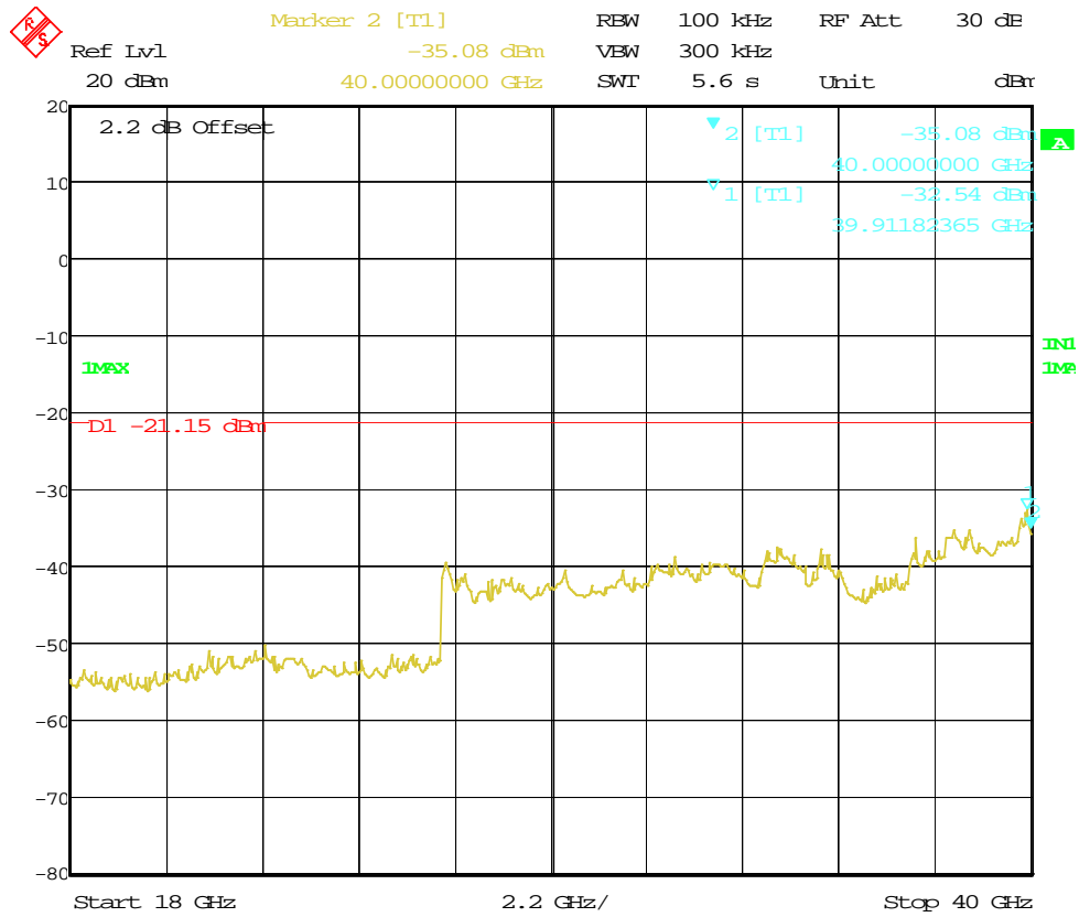
Figure 84: Out of Band Emission for HT20 at 5785 MHz, Chain 3
