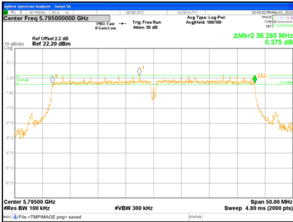
Figure 53: DTS Bandwidth at 5795 MHz, Chain 0
