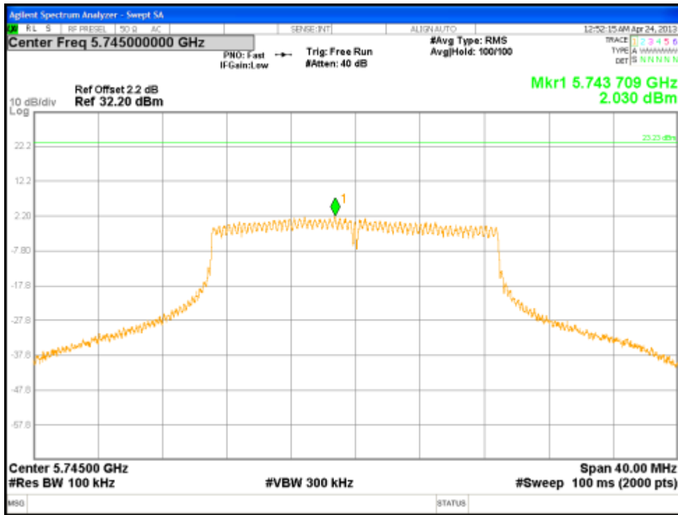
Figure 115: PPSD, 5745 MHz at 802.11n HT20, Chain 2 – 6.5 Mbps
