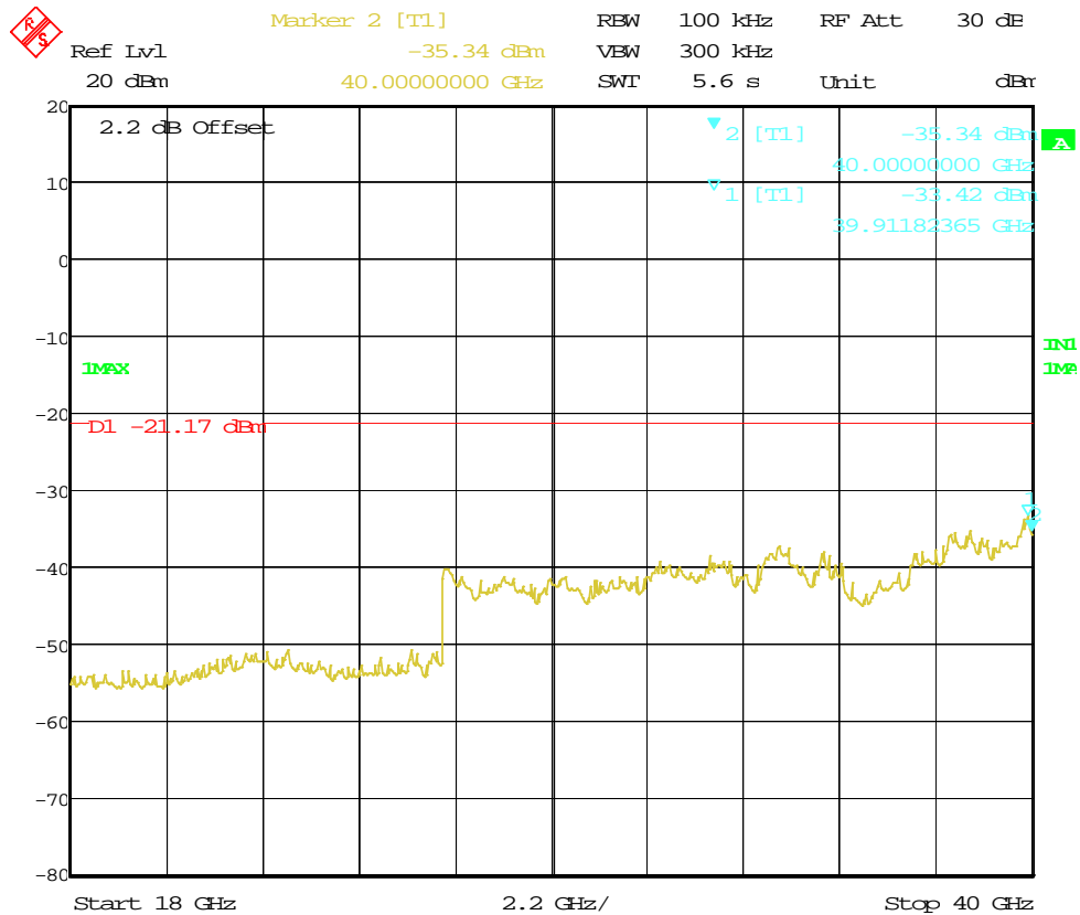
Figure 93: Out of Band Emission for HT20 at 5825 MHz, Chain 2
