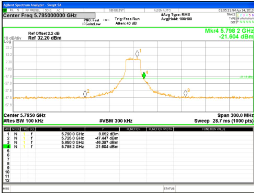
Figure 82: Reference Level for HT20 at 5785 MHz, Chain 3
