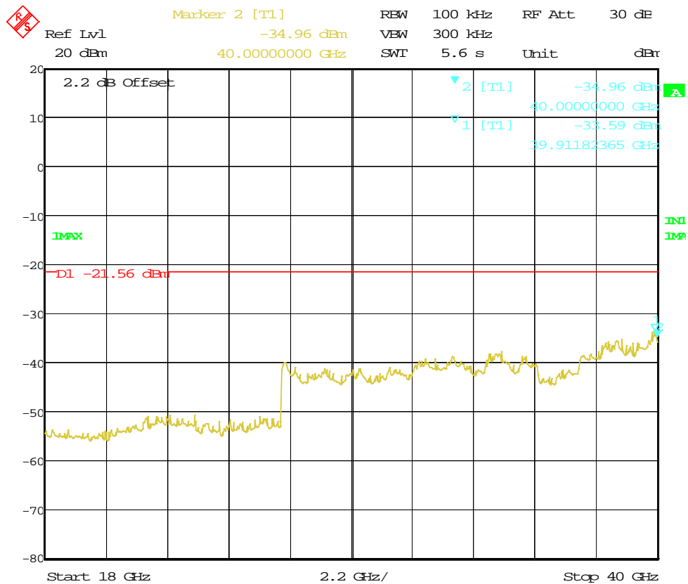
Figure 81: Out of Band Emission for HT20 at 5785 MHz, Chain 2
