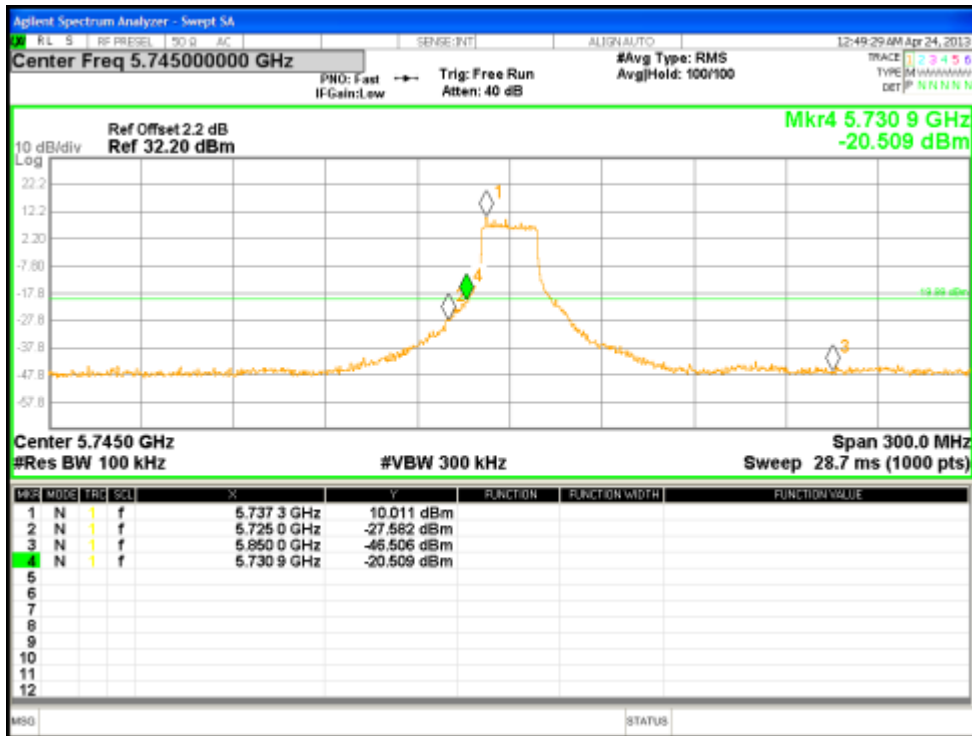
Figure 64: Reference Level for HT20 at 5745 MHz, Chain 1
