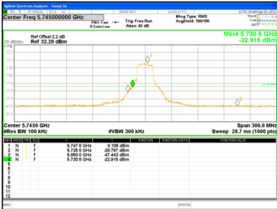
Figure 67: Reference Level for HT20 at 5745 MHz, Chain 2
