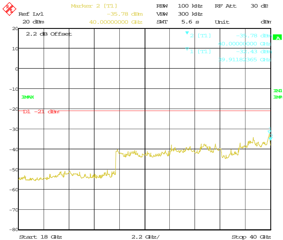
Figure 87: Out of Band Emission for HT20 at 5825 MHz, Chain 0
