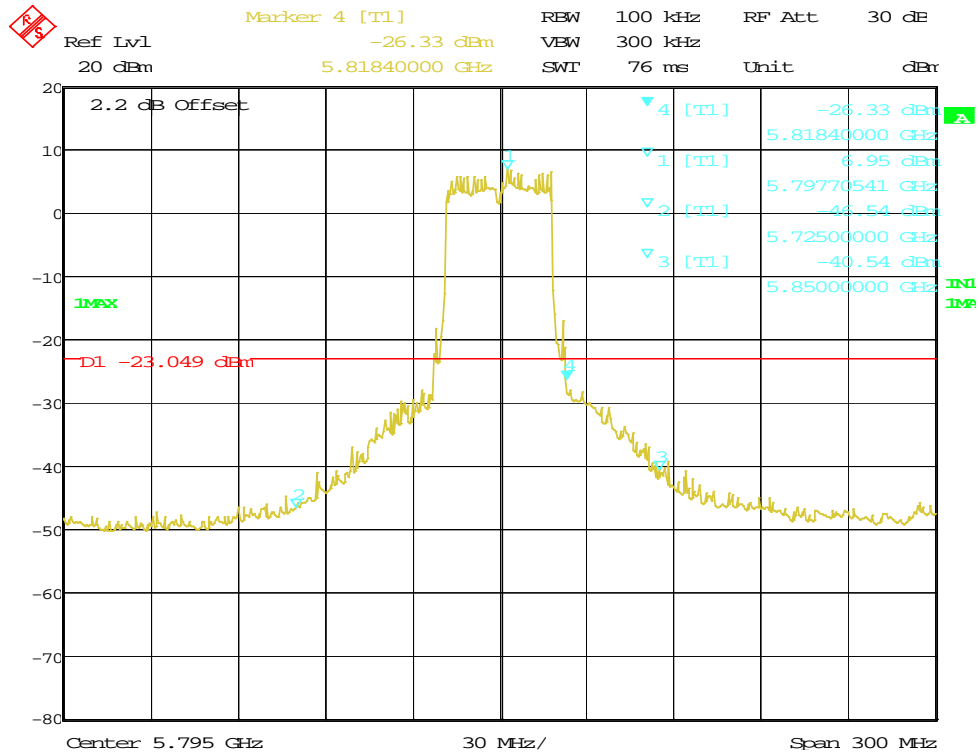
Figure 105: Reference Level for HT40 at 5795 MHz, Chain 0
