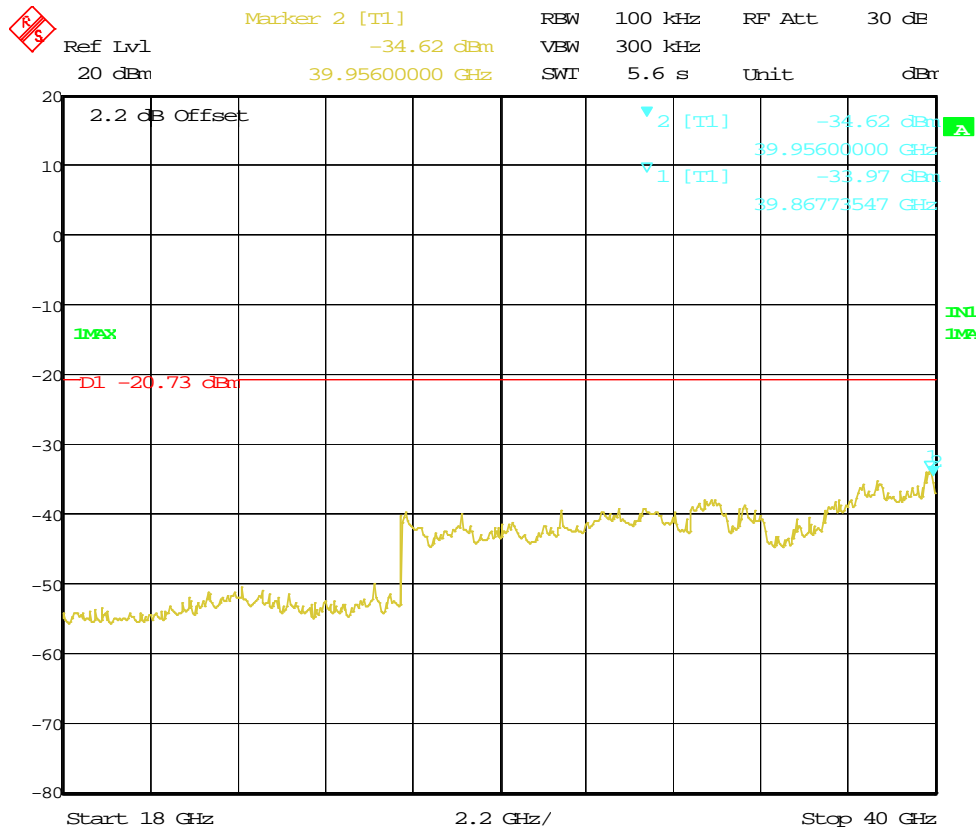
Figure 63: Out of Band Emission for HT20 at 5745 MHz, Chain 0
