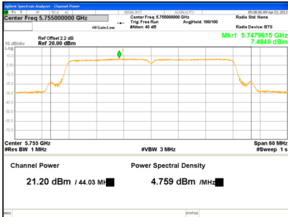
Figure 14: Maximum Transmitted Power, 5755MHz at HT40, Chain 1
