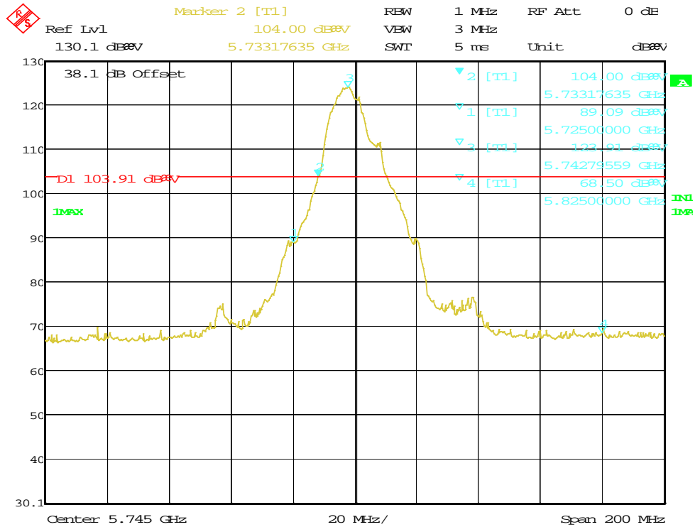
Figure 133: Radiated Emission at the Edge for 5745 MHz – Horiz. (Pk)
