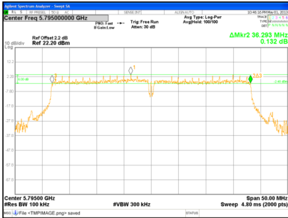
Figure 57: DTS Bandwidth at 5795 MHz, Chain 2
