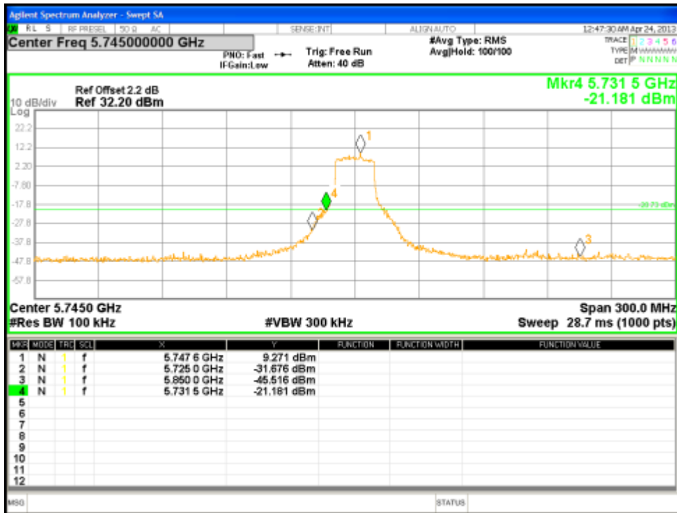
Figure 61: Reference Level for HT20 at 5745 MHz, Chain 0
