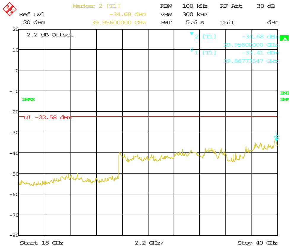
Figure 96: Out of Band Emission for HT20 at 5825 MHz, Chain 3
