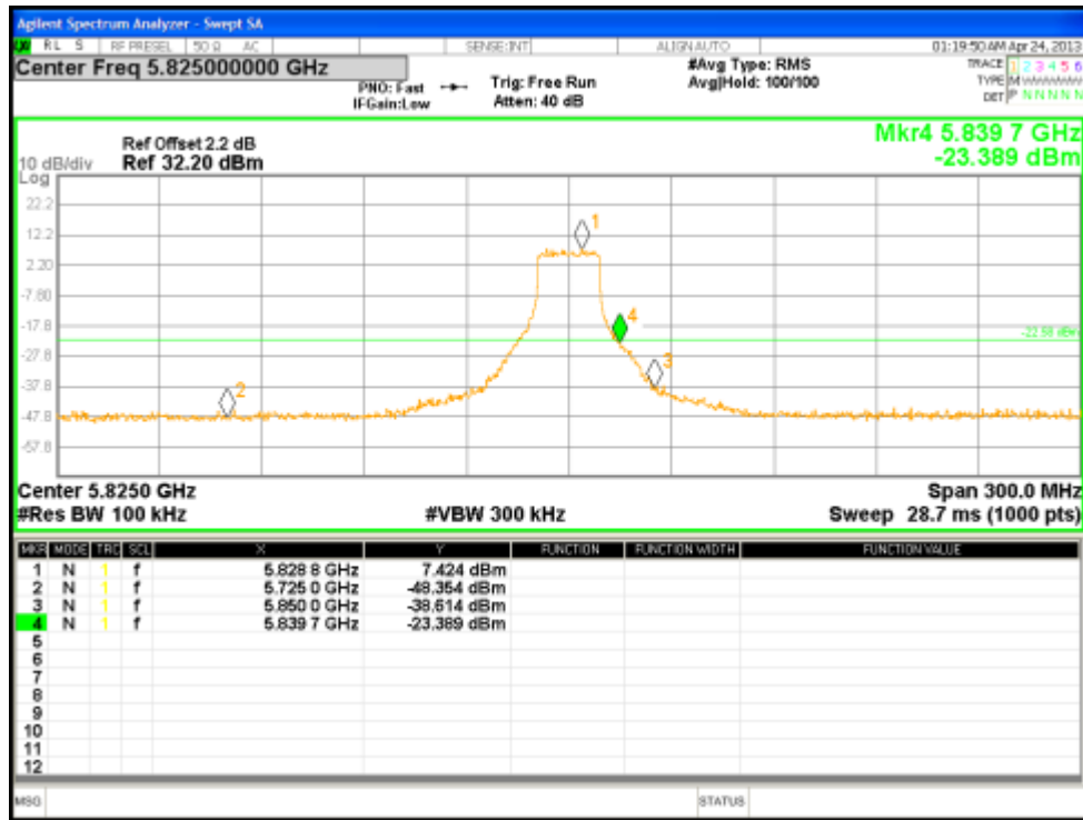
Figure 94: Reference Level for HT20 at 5825 MHz, Chain 3
