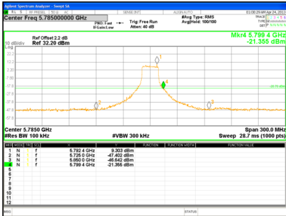
Figure 76: Reference Level for HT20 at 5785 MHz, Chain 1
