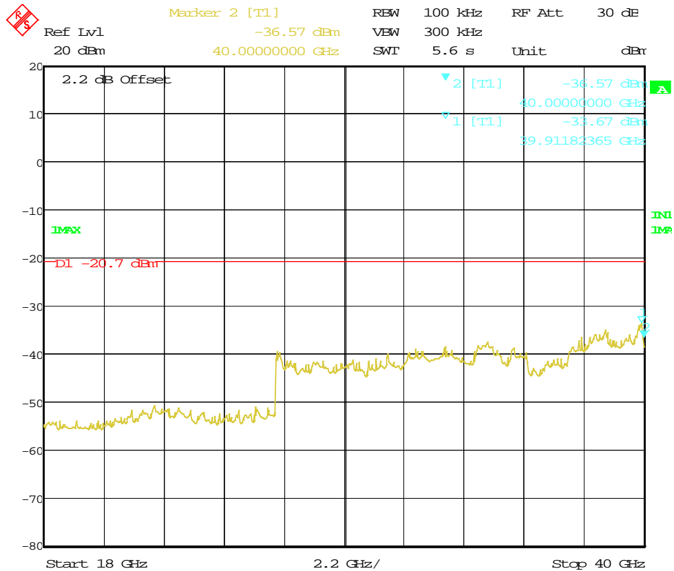
Figure 78: Out of Band Emission for HT20 at 5785 MHz, Chain 1
