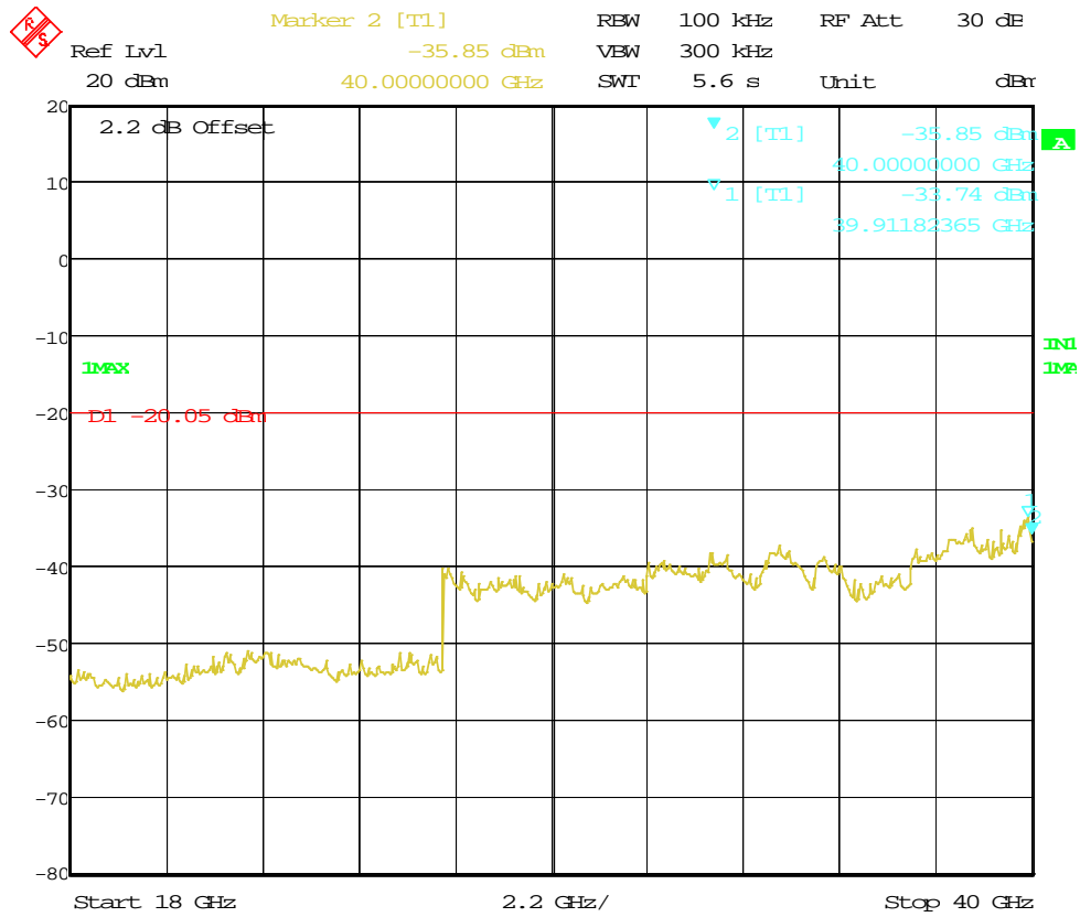
Figure 90: Out of Band Emission for HT20 at 5825 MHz, Chain 1
