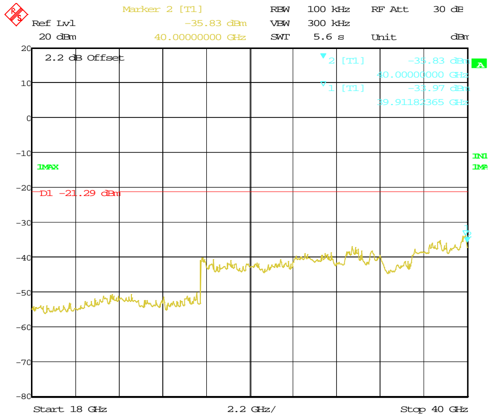
Figure 72: Out of Band Emission for HT20 at 5745 MHz, Chain 3
