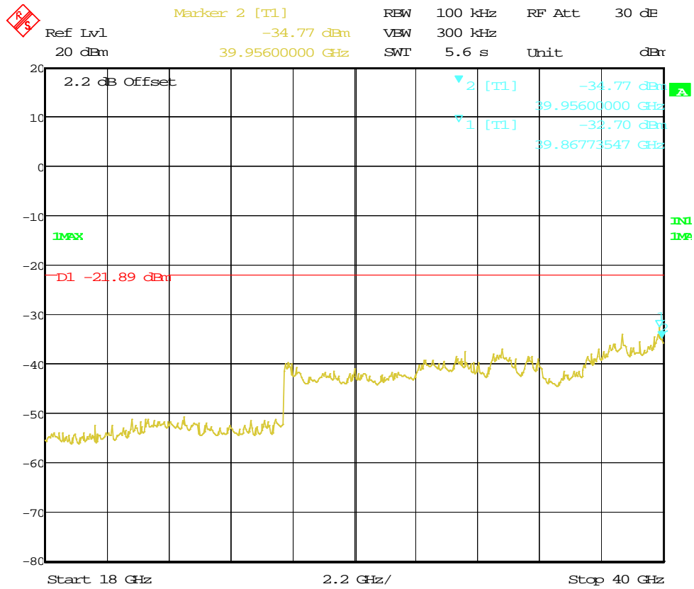
Figure 69: Out of Band Emission for HT20 at 5745 MHz, Chain 2
