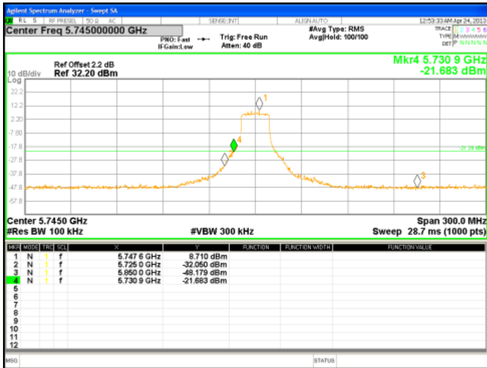
Figure 70: Reference Level for HT20 at 5745 MHz, Chain 3
