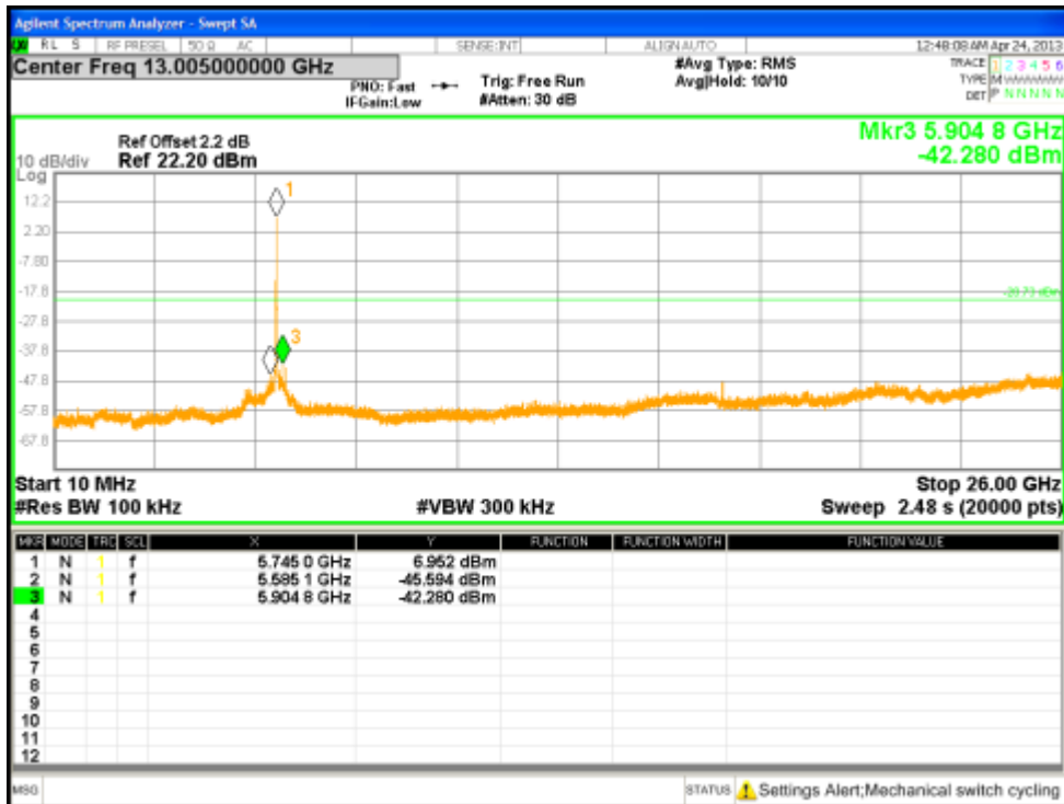
Figure 62: Out of Band Emission for HT20 at 5745 MHz, Chain 0
