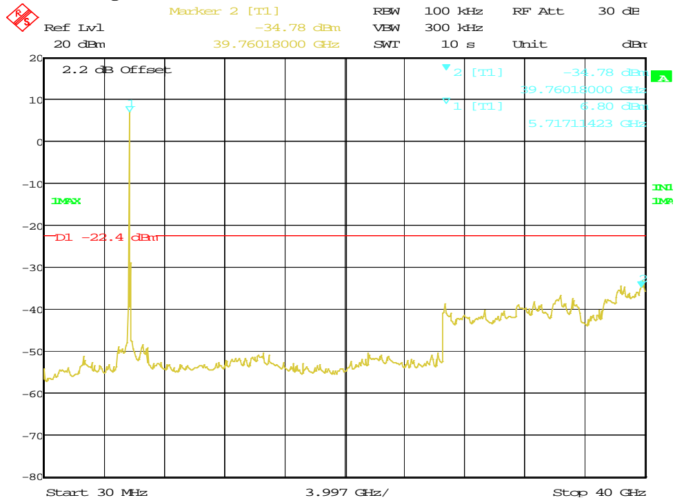
Figure 102: Out of Band Emission for HT40 at 5755 MHz, Chain 2
