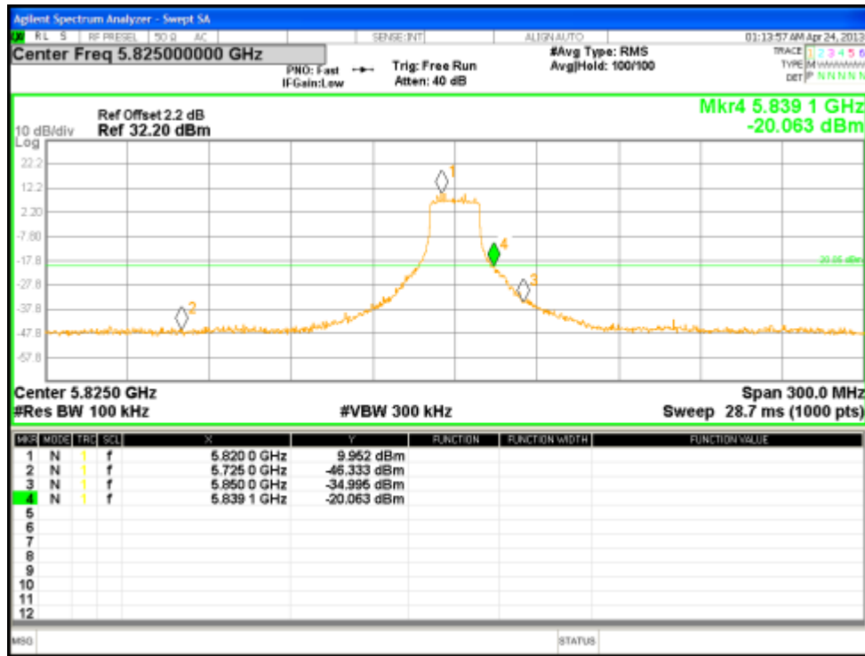
Figure 88: Reference Level for HT20 at 5825 MHz, Chain 1
