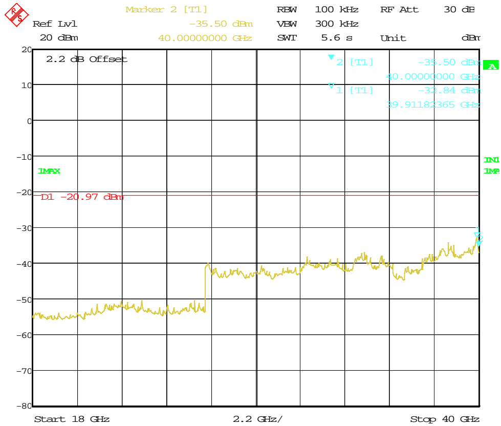
Figure 75: Out of Band Emission for HT20 at 5785 MHz, Chain 0
