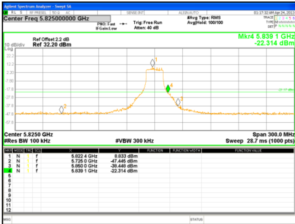
Figure 91: Reference Level for HT20 at 5825 MHz, Chain 2
