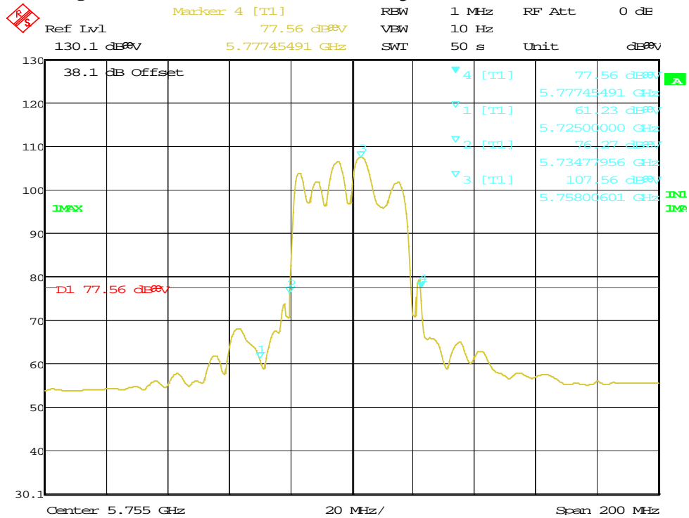
Figure 144: Radiated Emission at the Edge for 5755 MHz – Vert. (QP)
