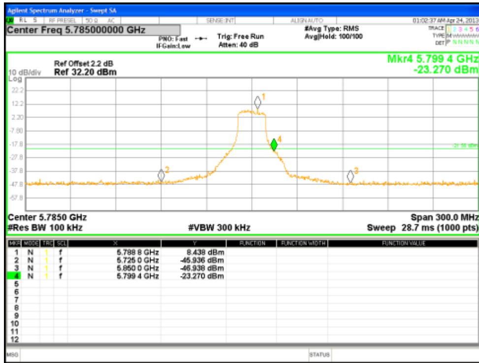
Figure 79: Reference Level for HT20 at 5785 MHz, Chain 2
