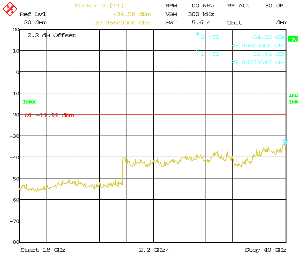
Figure 66: Out of Band Emission for HT20 at 5745 MHz, Chain 1
