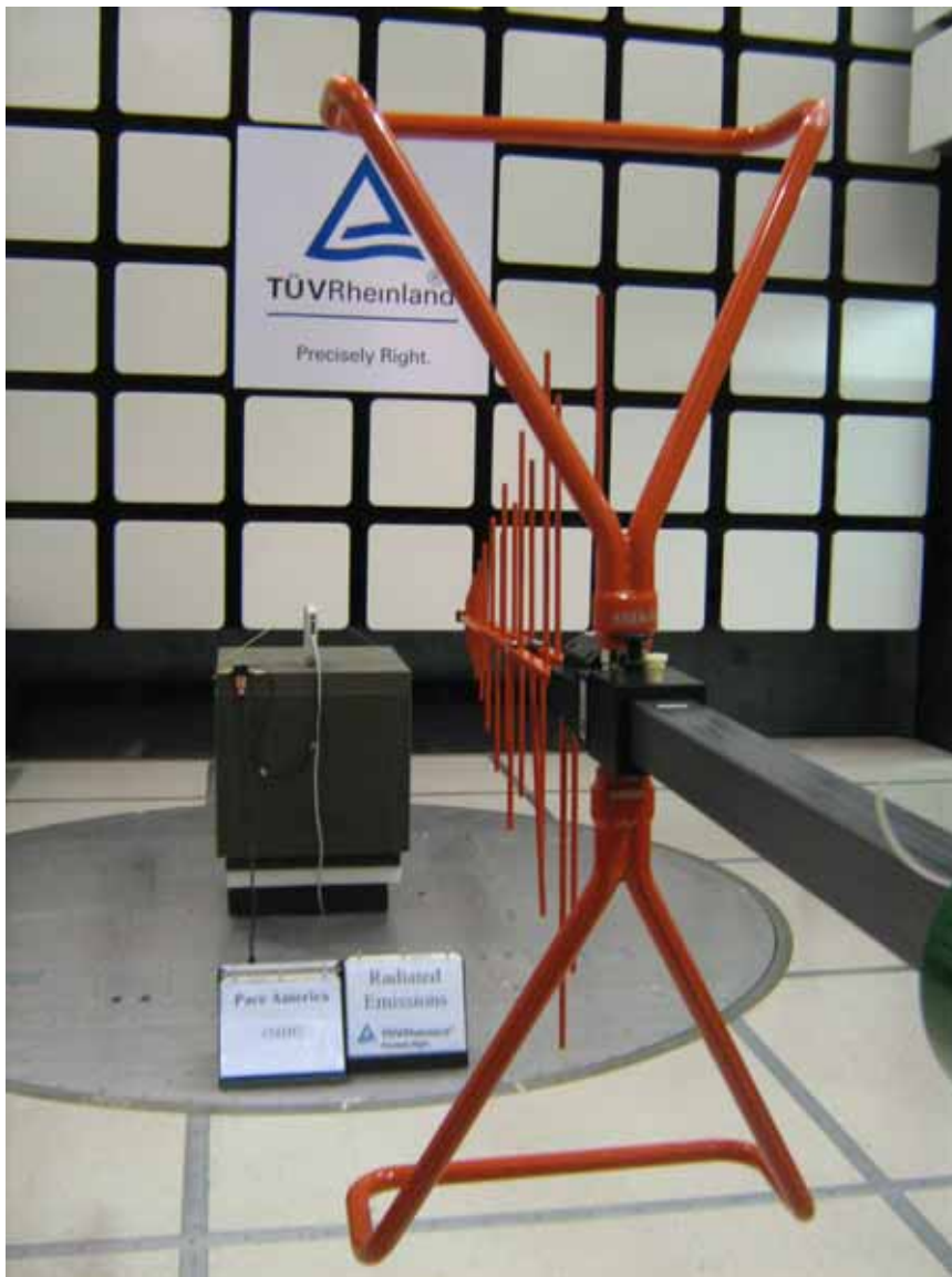
Figure 2: Test Setup for 30 MHz to 1000MHz (Rear View) – i38HG on Vertical Position
