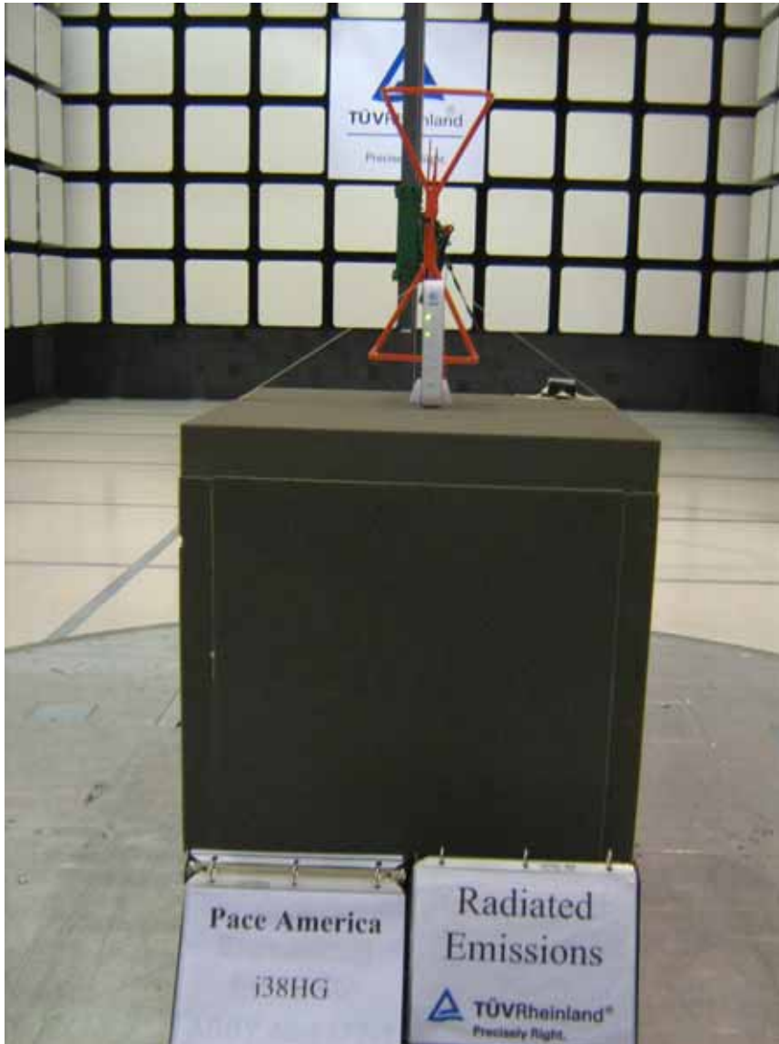
Figure 1: Test Setup for 30 MHz to 1000MHz (Front View) – i38HG on Vertical Position
