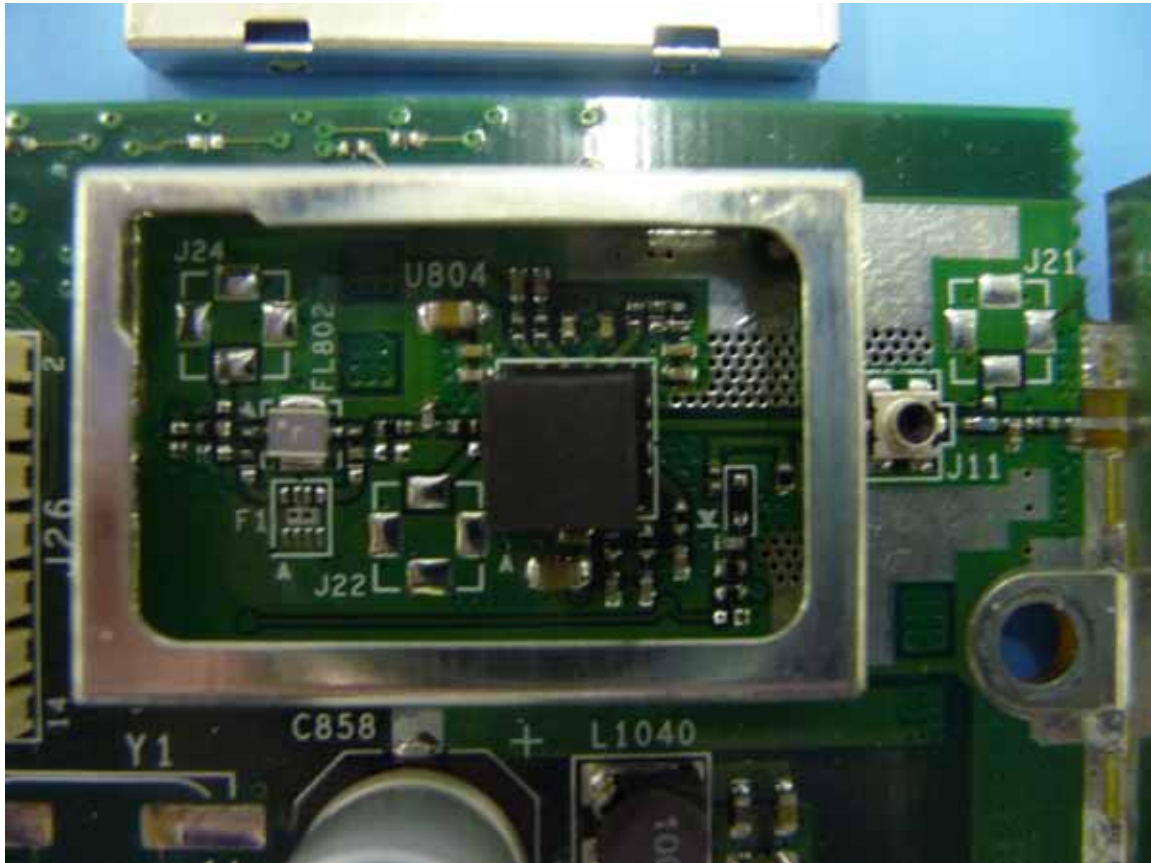
Figure 4: Internal Photo of I38HG – Inside the Chipset RF Can.
