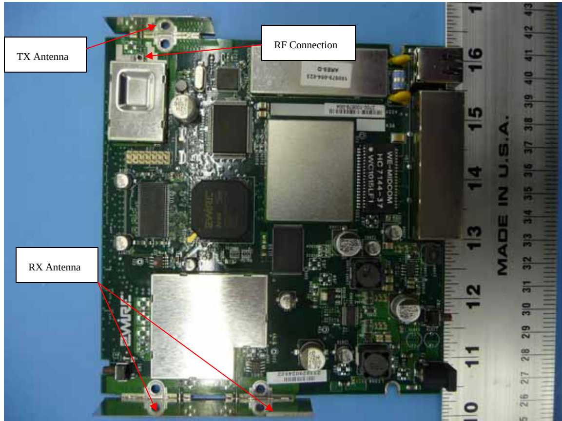
Figure 1: Internal Photo of i38HG - PCB Board (Front Side)
