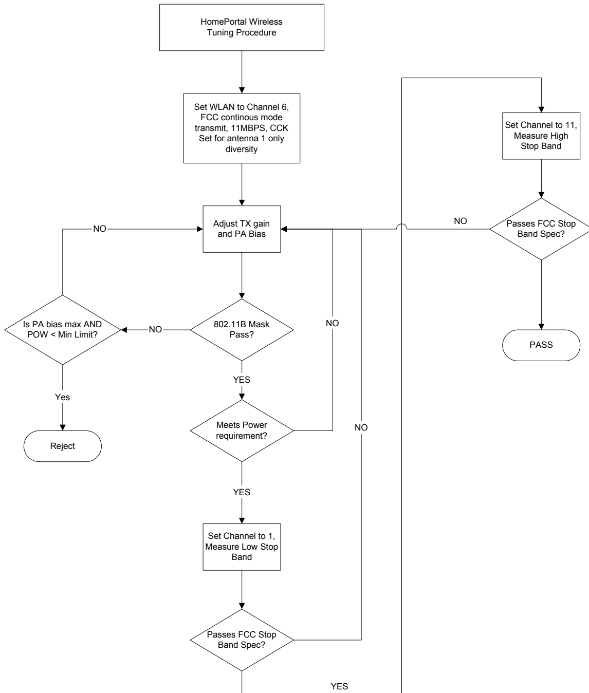
Figure 1 – Tuning Flowchart
