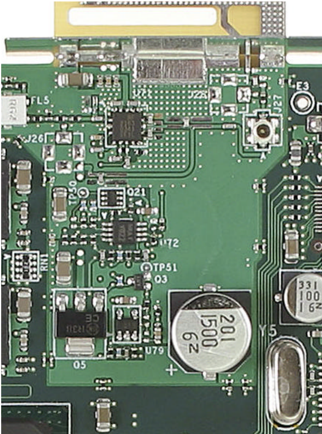
RF Amplifier Circuit Photo
