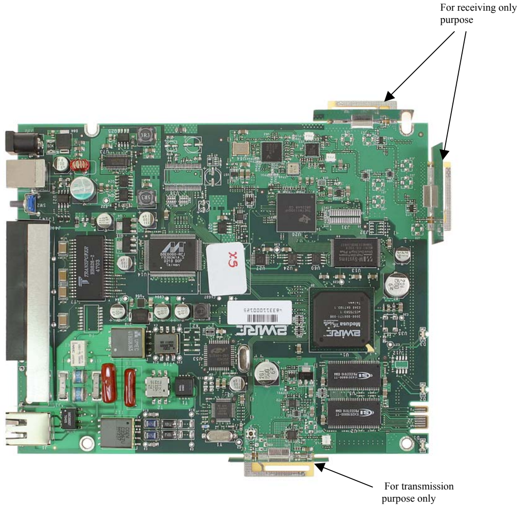
Figure 4 - Main Board, Top View
