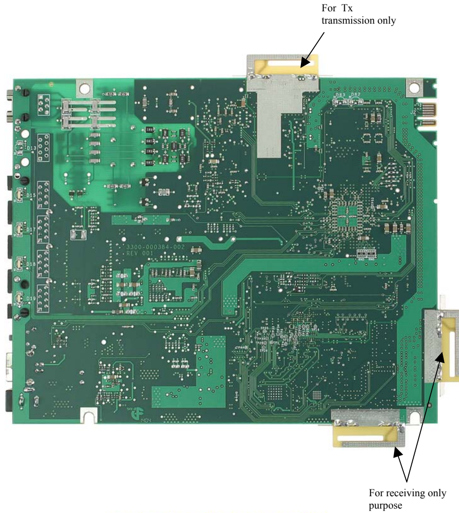
Figure 5 - Main Board, Bottom View
