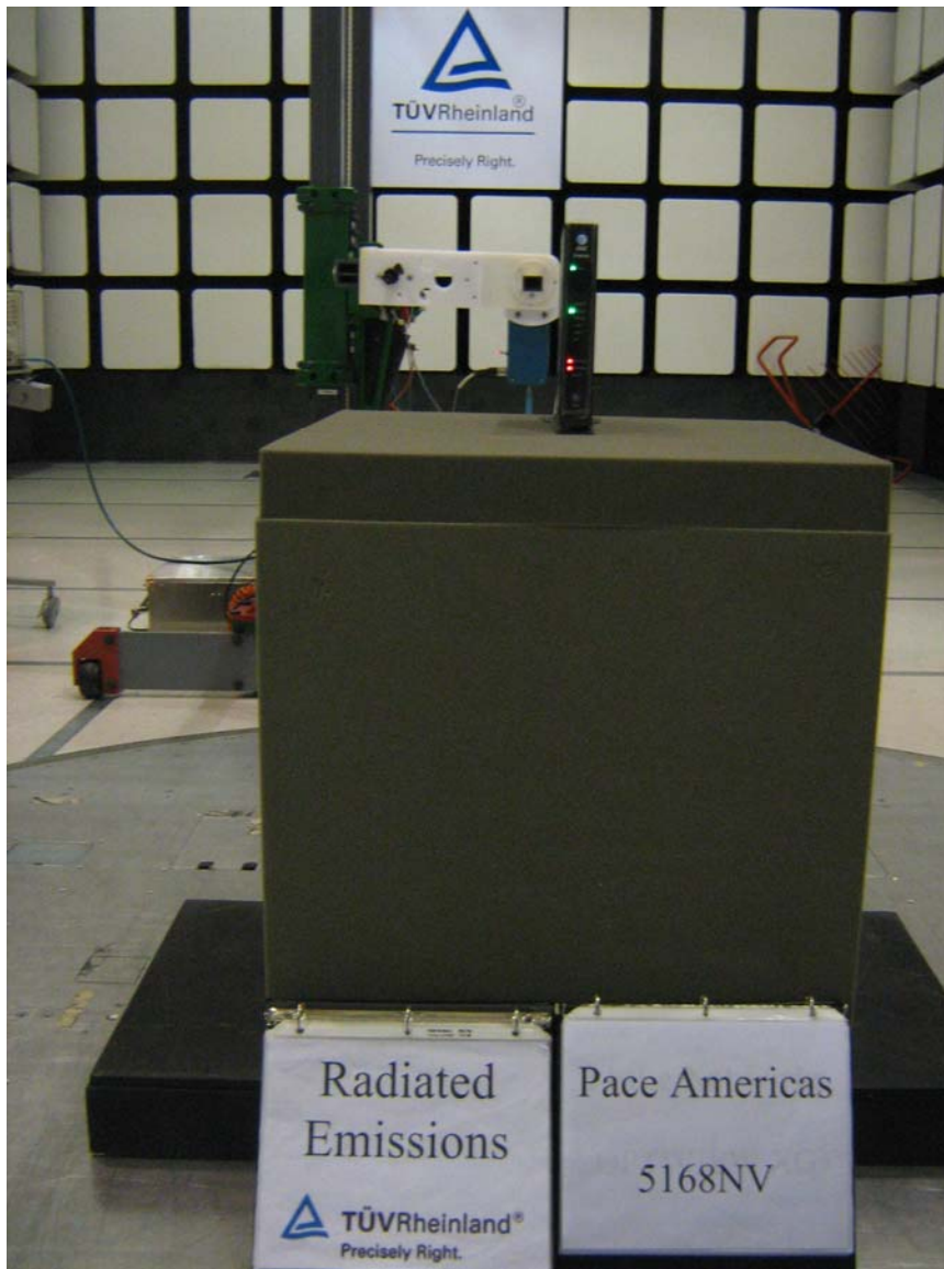
Figure 5: Test Setup for 18 GHz to 26GHz (Front View) – 5168NV on Vertical Position
