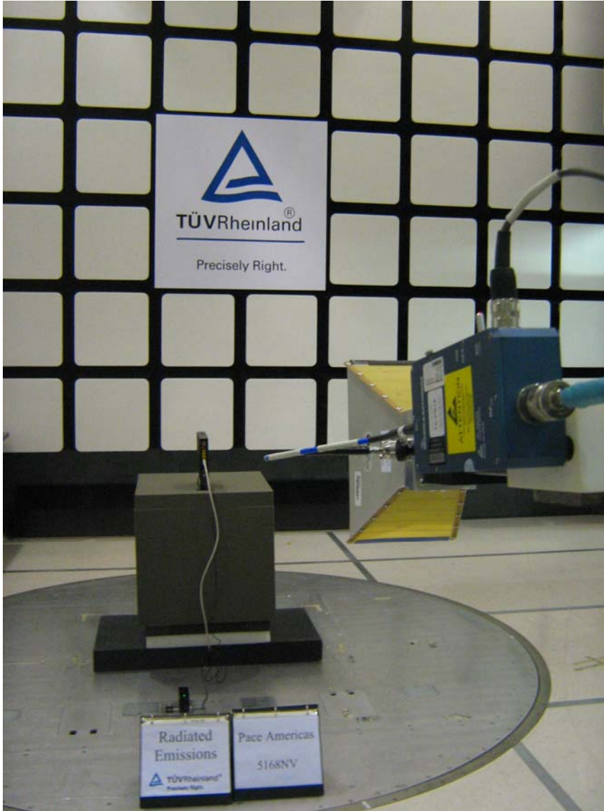
Figure 4: Test Setup for 1GHz to 18GHz (Rear View) – 5168NV on Vertical Position
