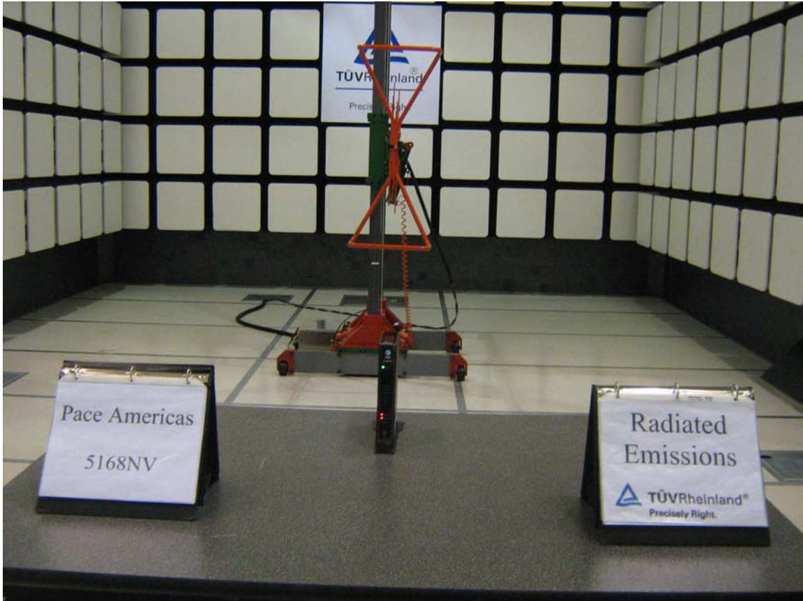
Figure 1: Test Setup for 30 MHz to 1000MHz (Front View) – 5168NV on Vertical Position
