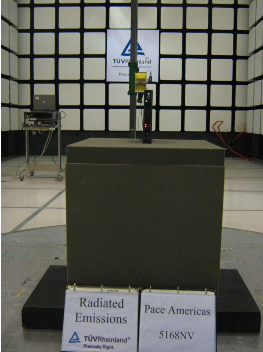
Figure 3: Test Setup for 1GHz to 18GHz (Front View) – 5168NV on Vertical Position
