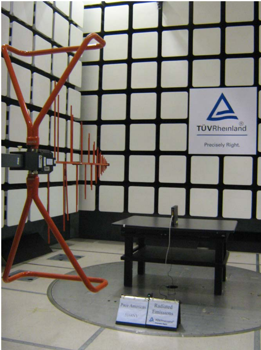
Figure 2: Test Setup for 30 MHz to 1000MHz (Rear View) – 5168NV on Vertical Position
