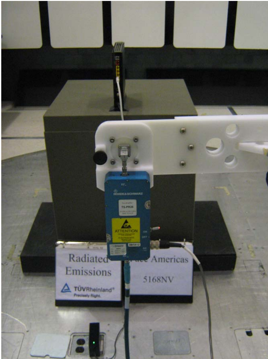
Figure 6: Test Setup for 18 GHz to 26GHz (Rear View) - 5168NV on Vertical Position
