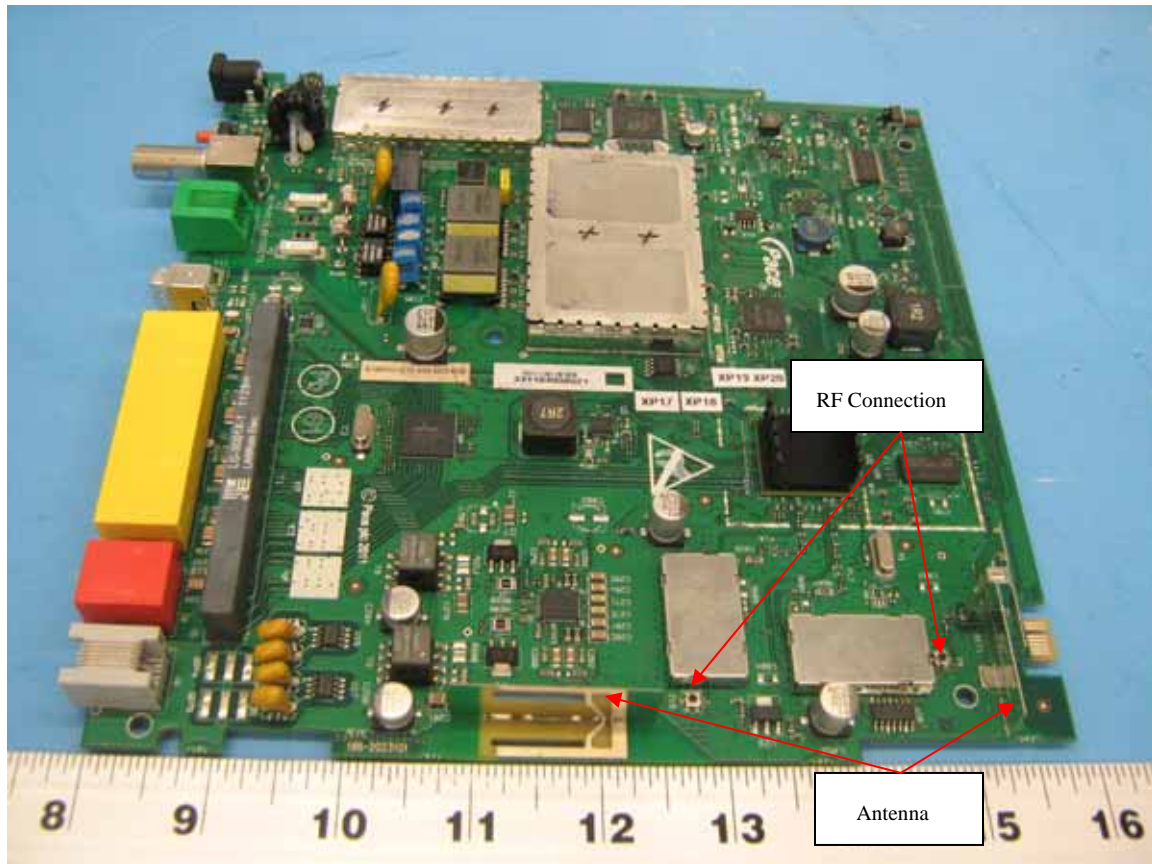
Figure 1: Internal Photo of 5168 - PCB Board (Front Side)
