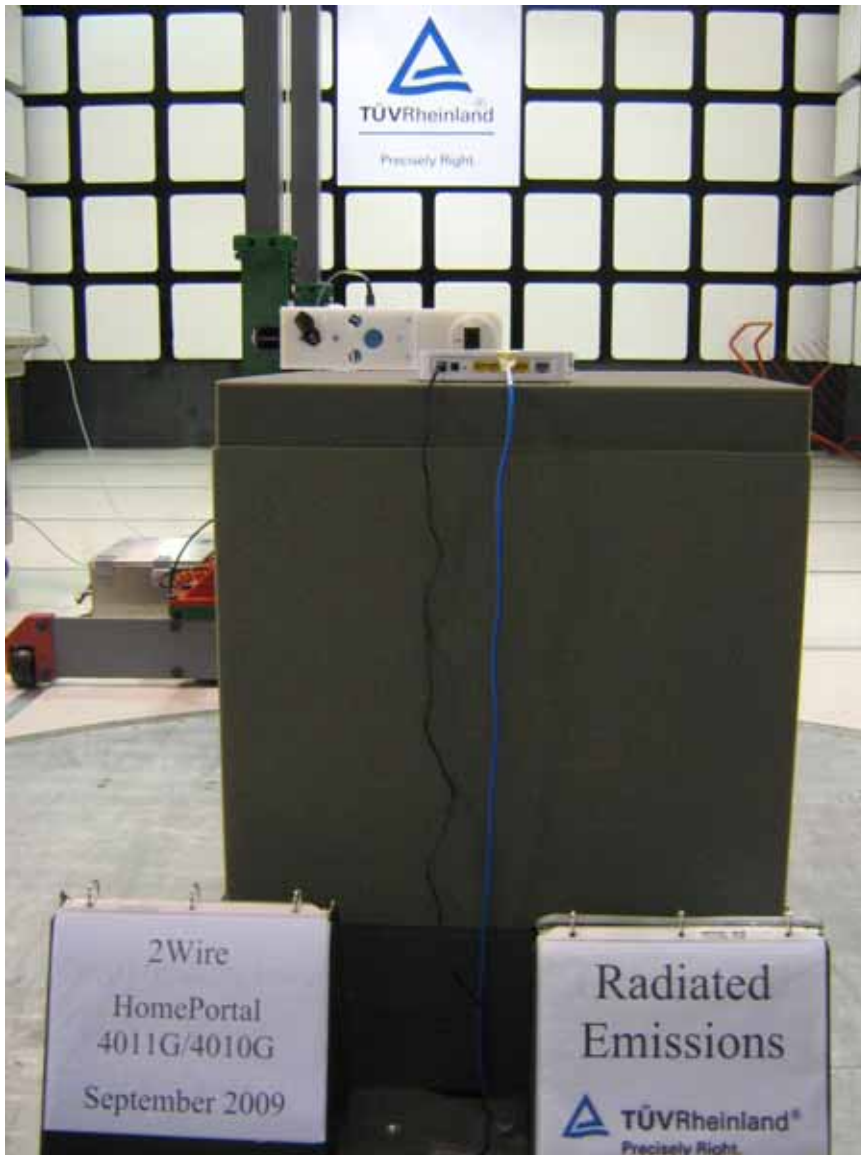
Figure 5: Photo of Test Setup for 4011G/4010G, 18 GHz to 26GHz (Front View)
