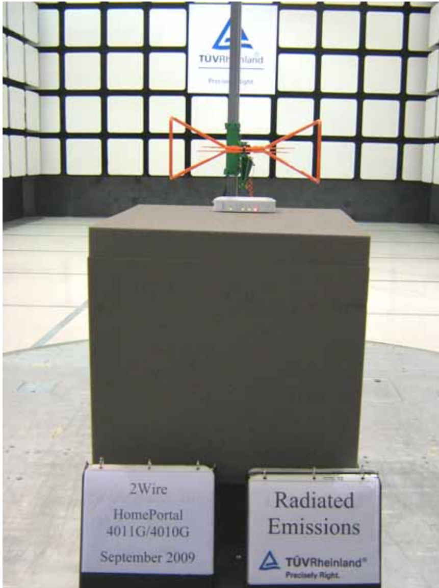
Figure 1: Photo of Test Setup for 4011G/4010G, 30 MHz to 1000MHz (Front View)
