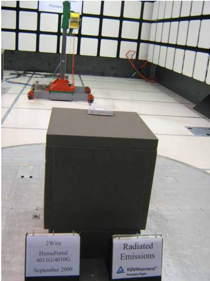
Figure 3: Photo of Test Setup for 4011G/4010G, 1GHz to 18GHz (Front View)
