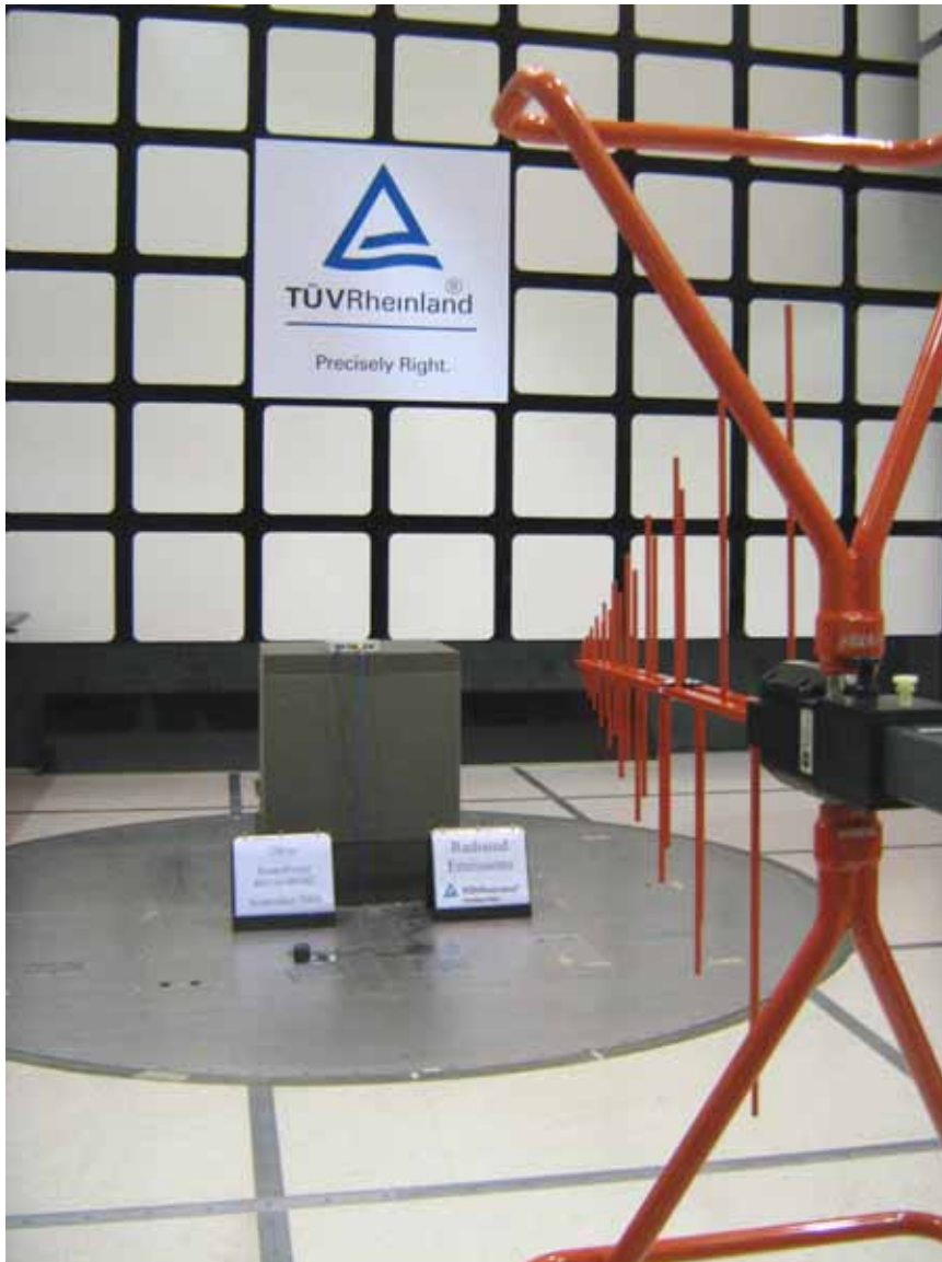
Figure 2: Photo of Test Setup for 4011G/4010G, 30 to 1000 MHz (Rear View)
