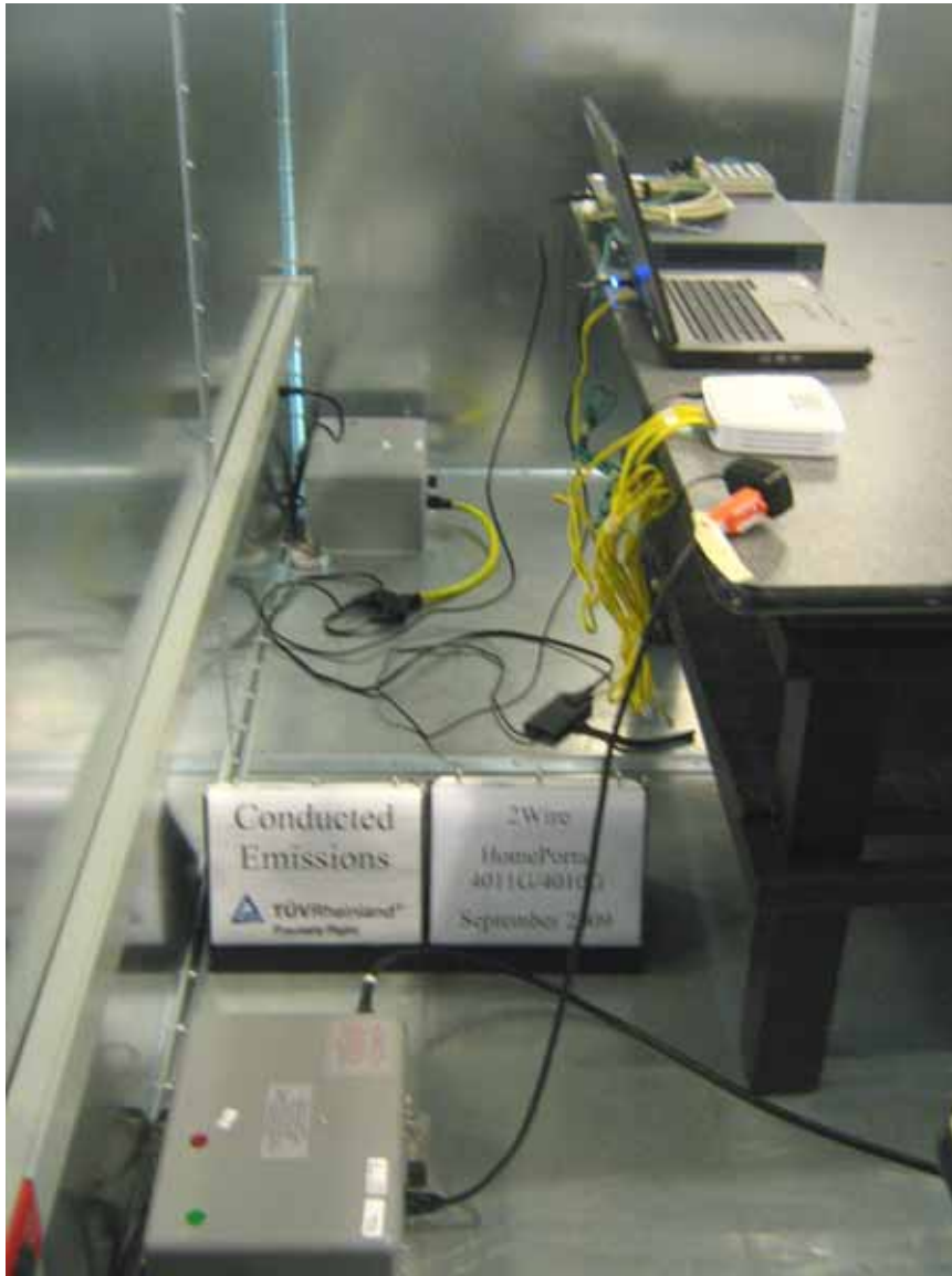
Figure 8: Photo of Test Setup for 4011G/4010G, AC Conducted Emission (Side View)
