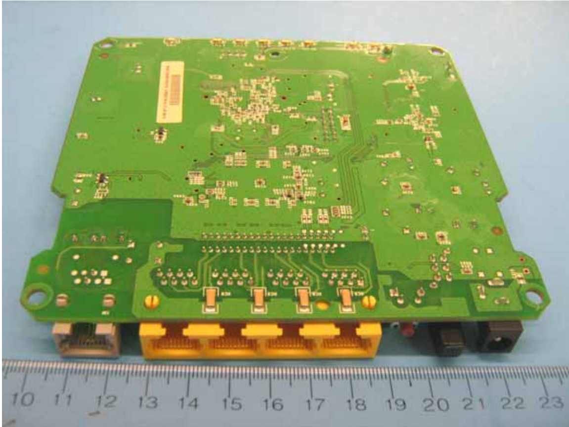
Figure 5: Internal Photo of 4011G/4010G - PCB Board (Rear Side)
