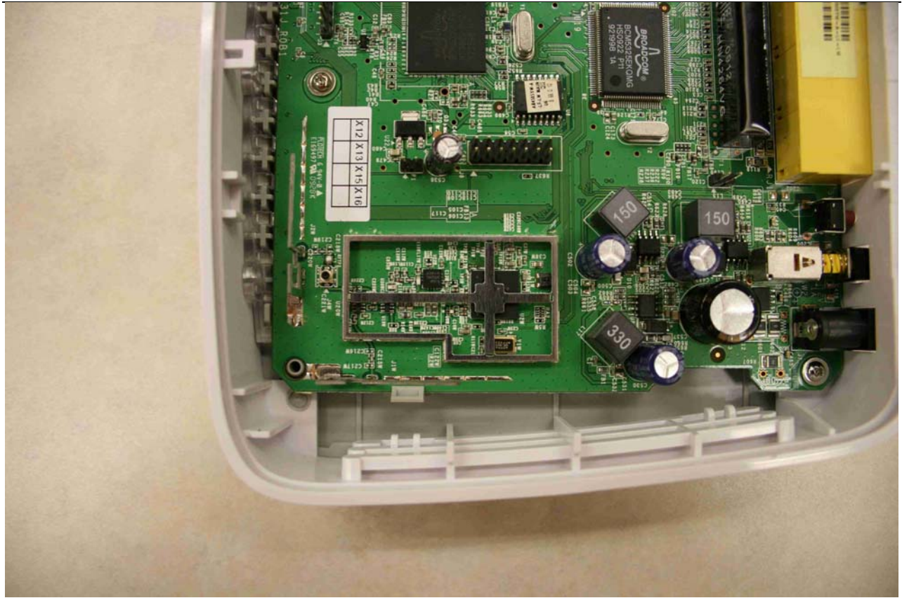
Figure 7: Internal Photo of 4011G/4010G - PCB Board with Shields OFF
