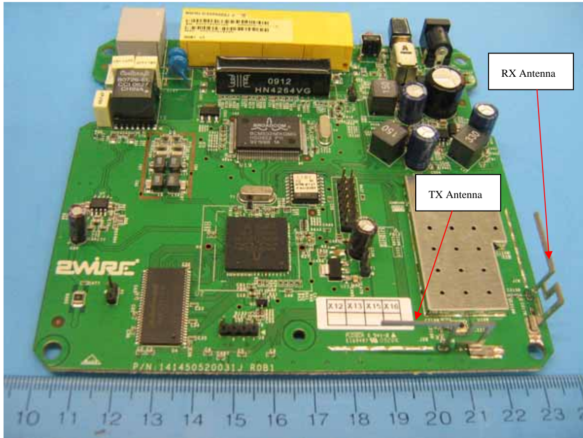
Figure 4: Internal Photo of 4011G/4010G - PCB Board (Front Side)
