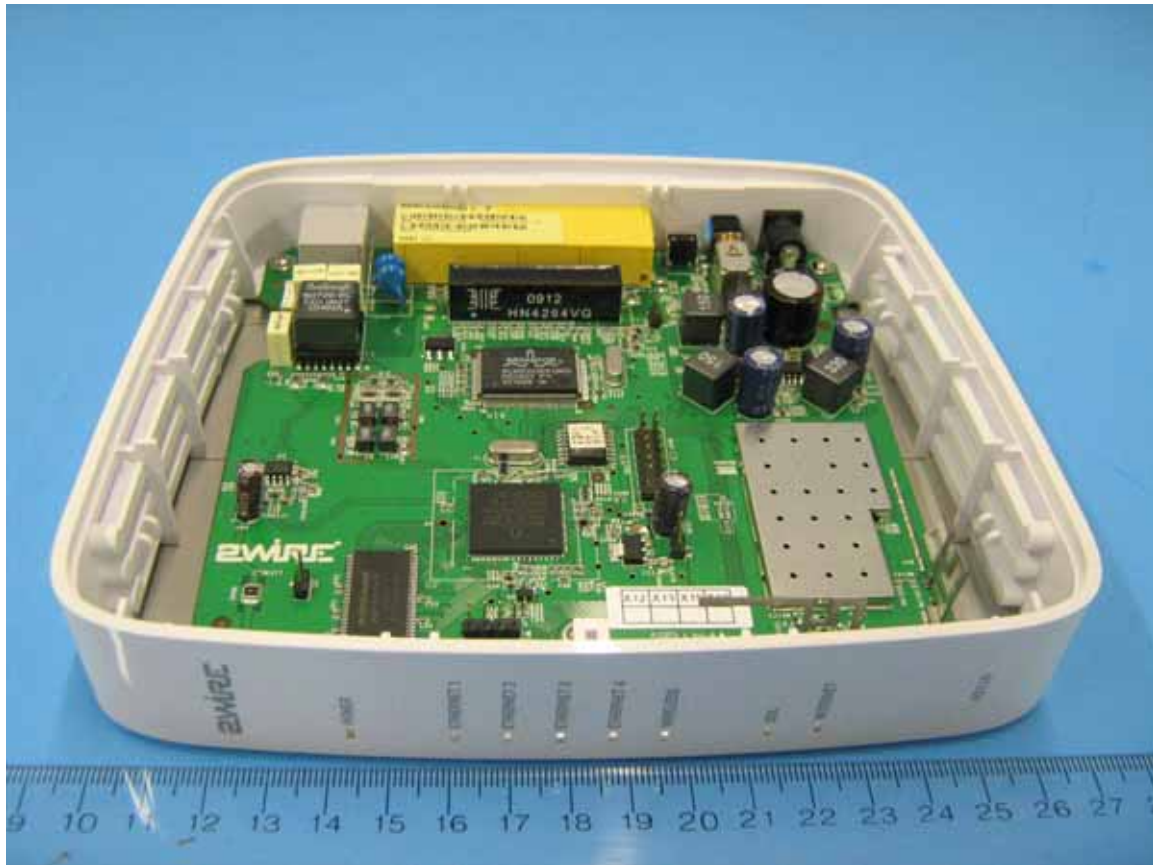
Figure 2: Photo of 4011G/4010G without Top Cover
