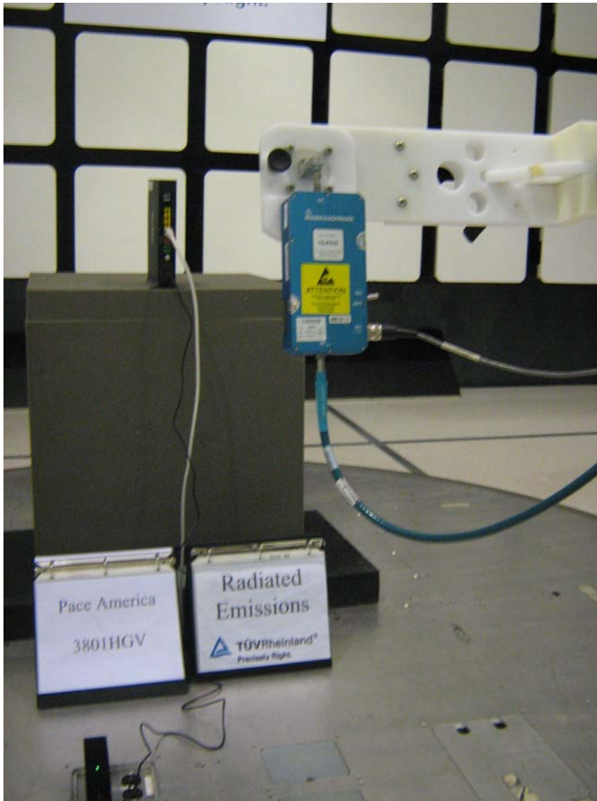
Figure 6: Test Setup for 18 GHz to 26GHz (Rear View) - 3801HGV on Vertical Position
