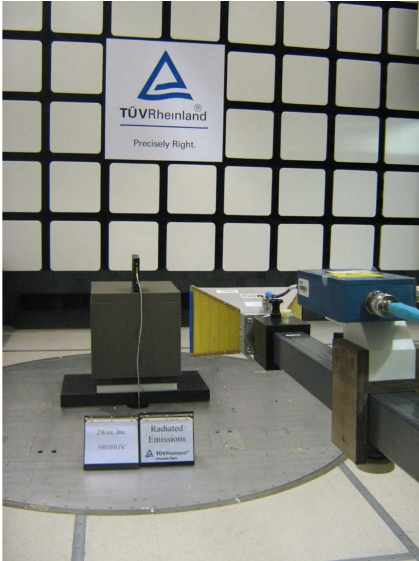
Figure 4: Test Setup for 1GHz to 18GHz (Rear View) - 3801HGV on Vertical Position
