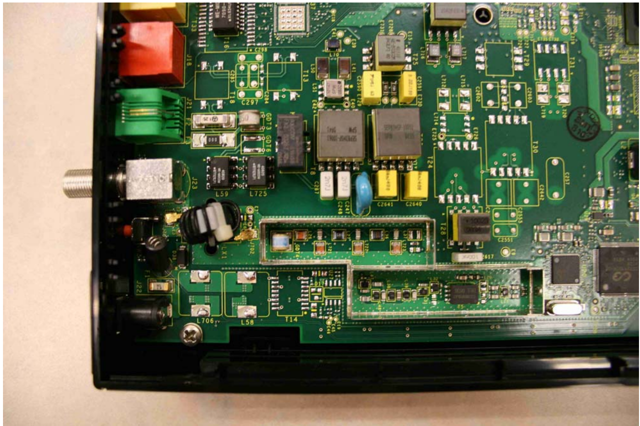
Figure 3: Internal Photo of HomePortal 3801HGV - PCB Shields removed
