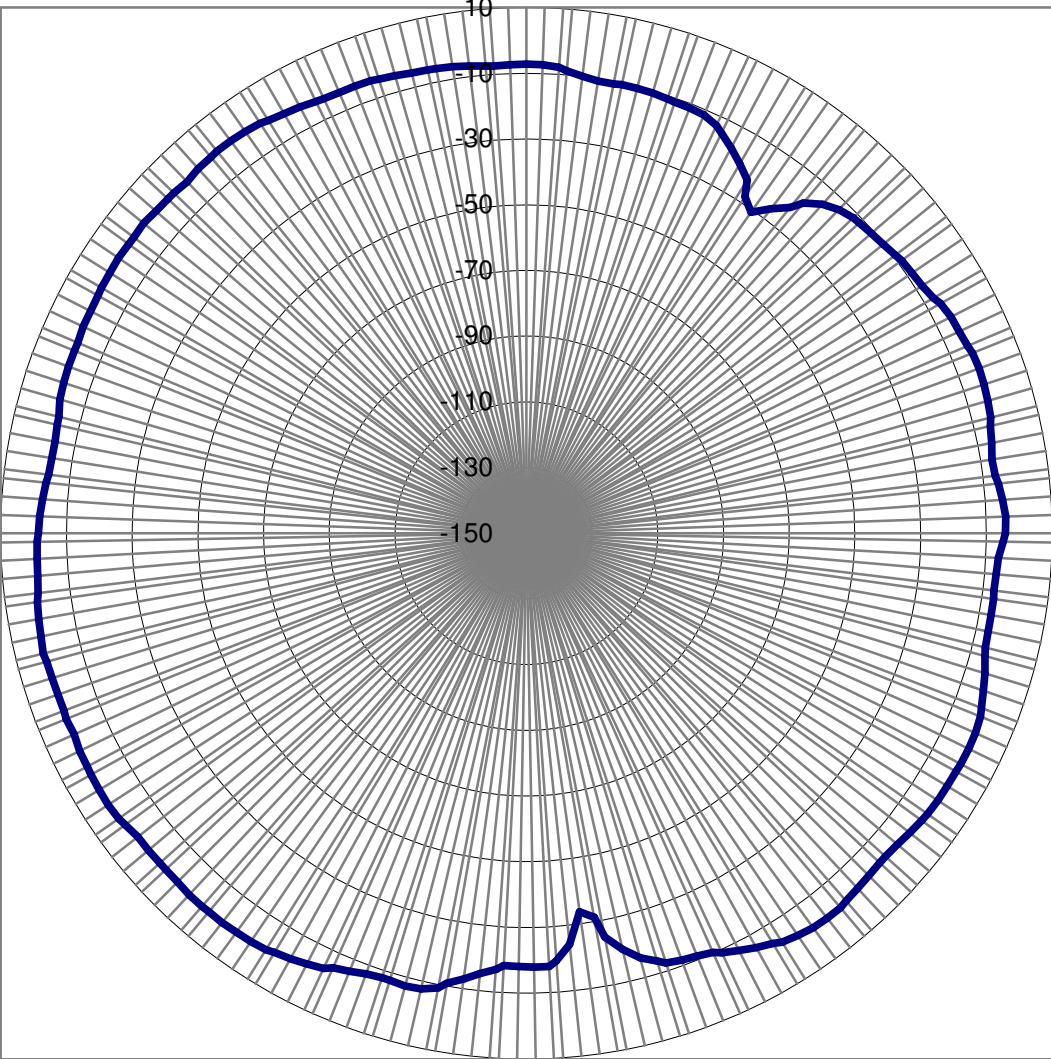
Polar Plot: Horizontal (EUT Standing)
