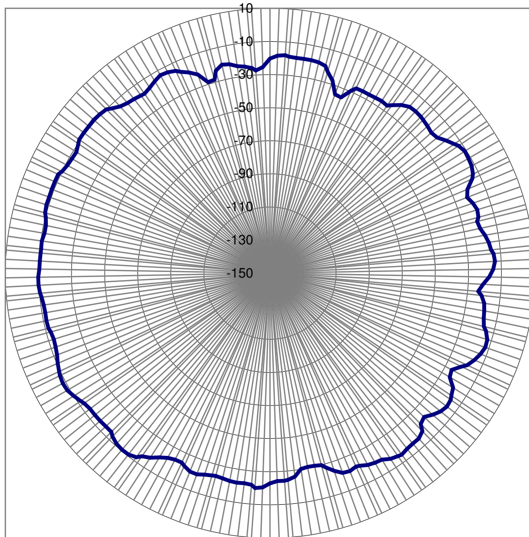
Polar Plot: Horizontal (EUT laying flat)
