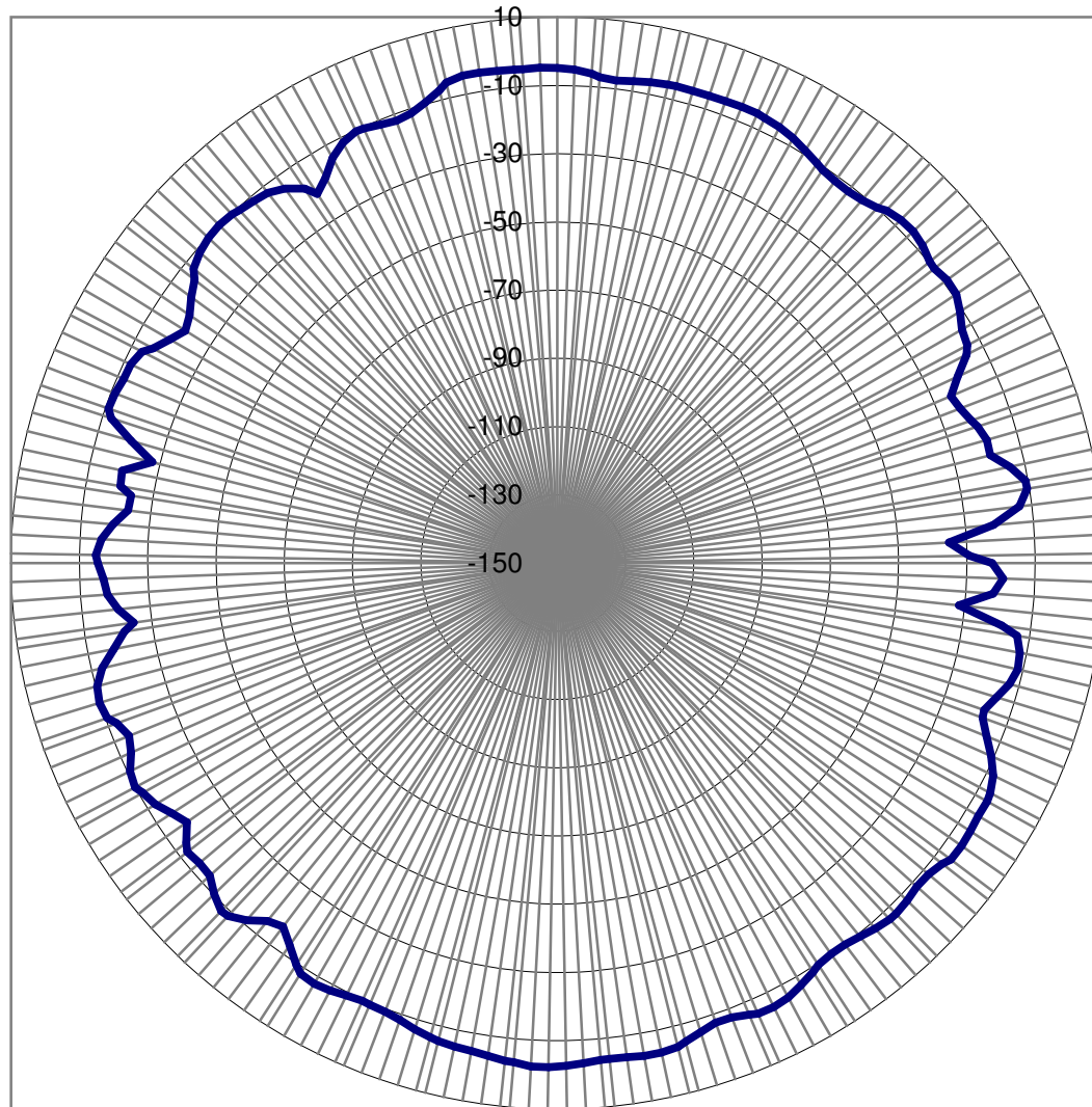
Polar Plot: Vertical (EUT laying flat)
