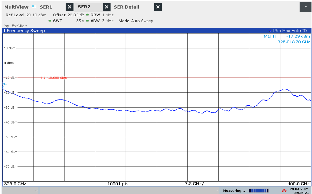
Plot 32: 325 GHz – 400 GHz, stopped mode (sweep stopped in the middle of the range of operation)
