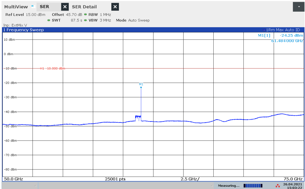
Plot 15: 50 GHz – 75 GHz, normal mode
