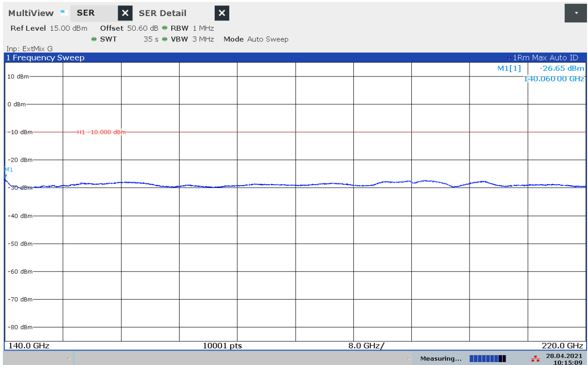
Plot 28: 140 GHz – 220 GHz, stopped mode (sweep stopped in the middle of the range of operation)
