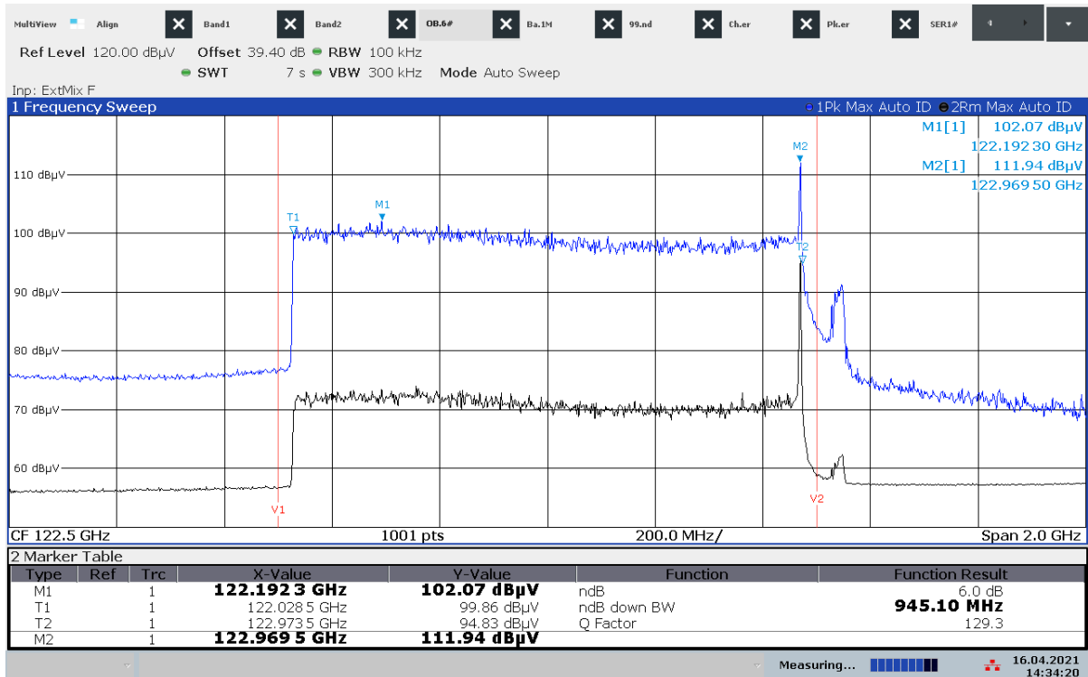
Plot 34: T_{min} / V_{nom}
