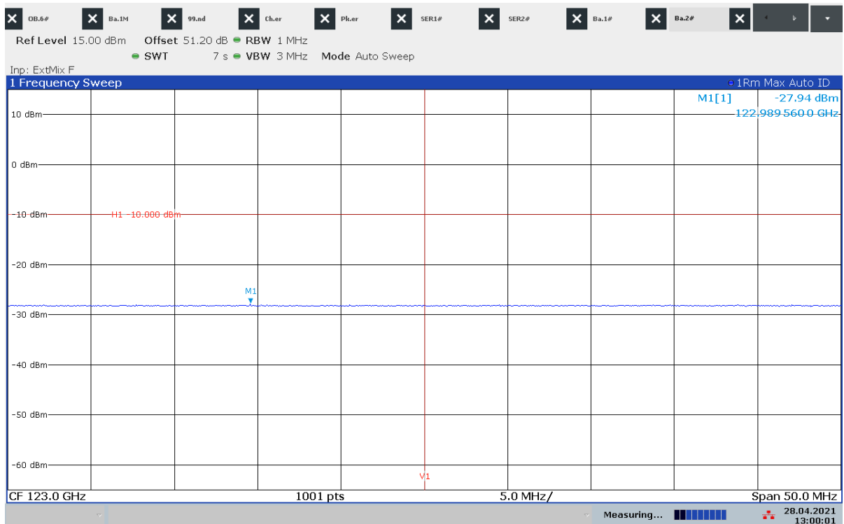
Plot 24: upper band edge compliance, stopped mode (sweep stopped in the middle of the range of operation)
