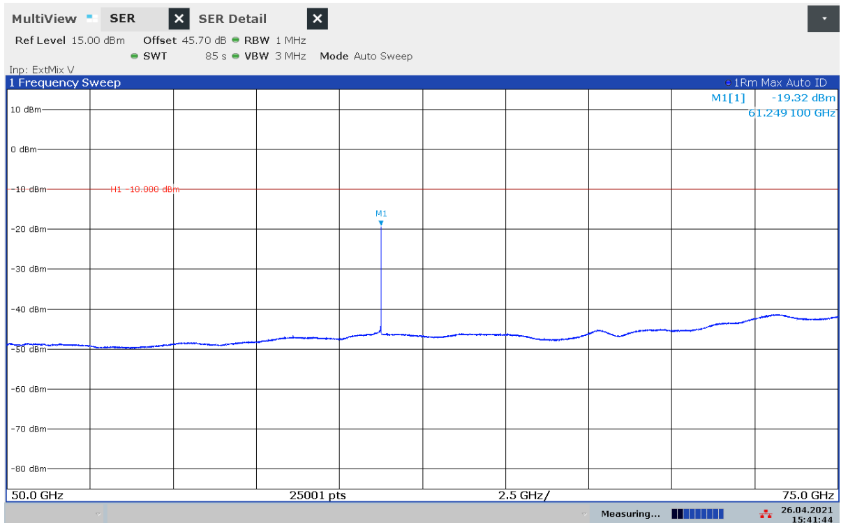
Plot 16: 50 GHz – 75 GHz, stopped mode (sweep stopped near the middle of the range of operation)
