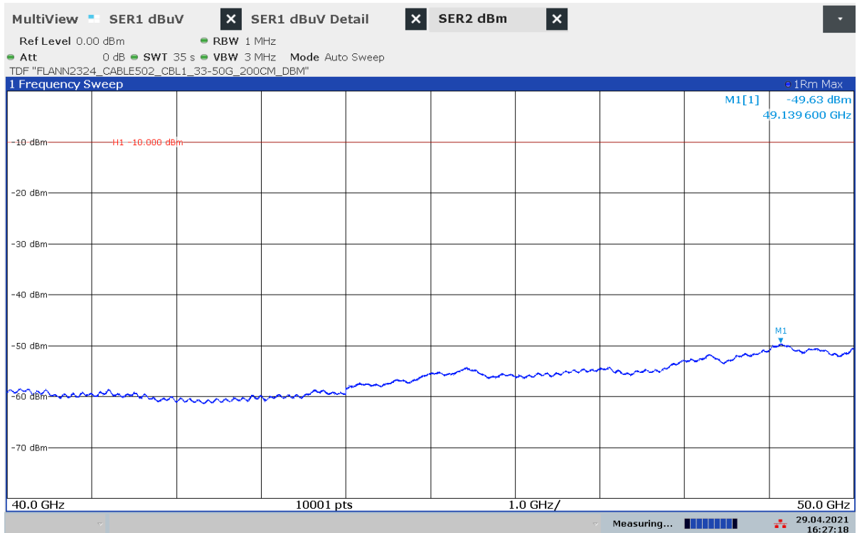
Plot 14: 40 GHz – 50 GHz, stopped mode (sweep stopped in the middle of the range of operation)
