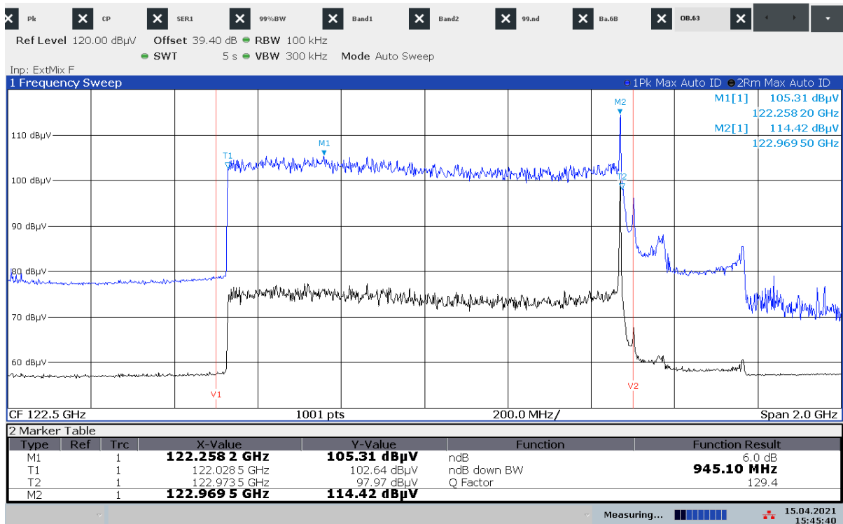
Plot 40: T_{min} / V_{nom}
