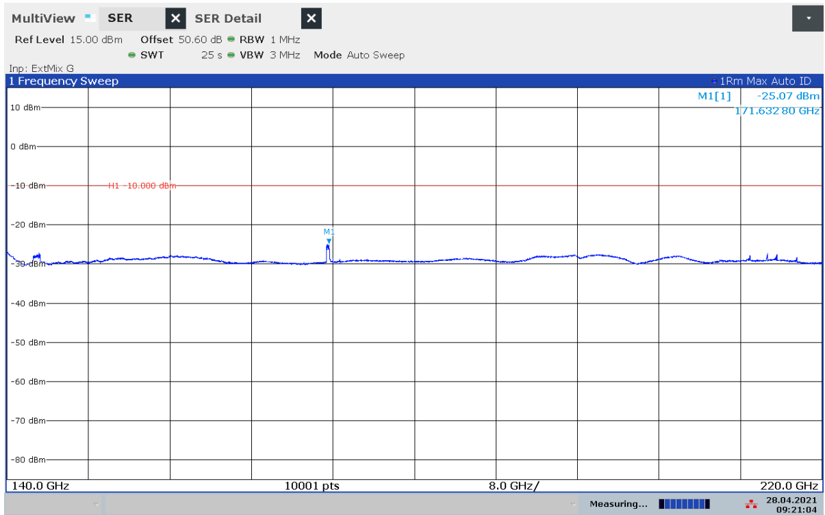
Plot 33: 140 GHz – 220 GHz, normal mode
