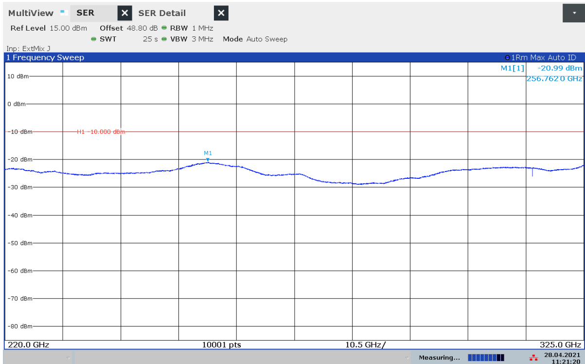
Plot 35: 220 GHz – 325 GHz, normal mode
