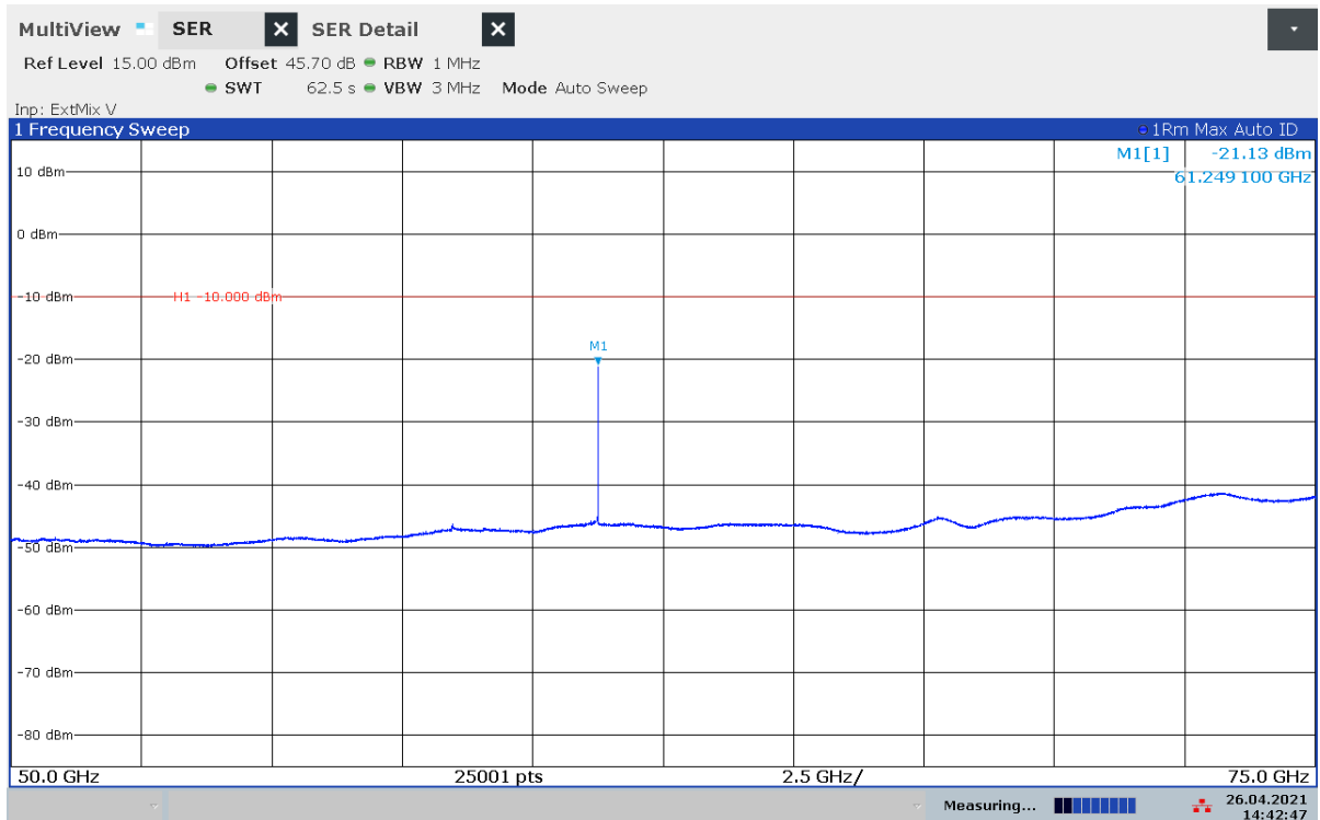
Plot 22: 50 GHz – 75 GHz, stopped mode (sweep stopped near the middle of the range of operation)
