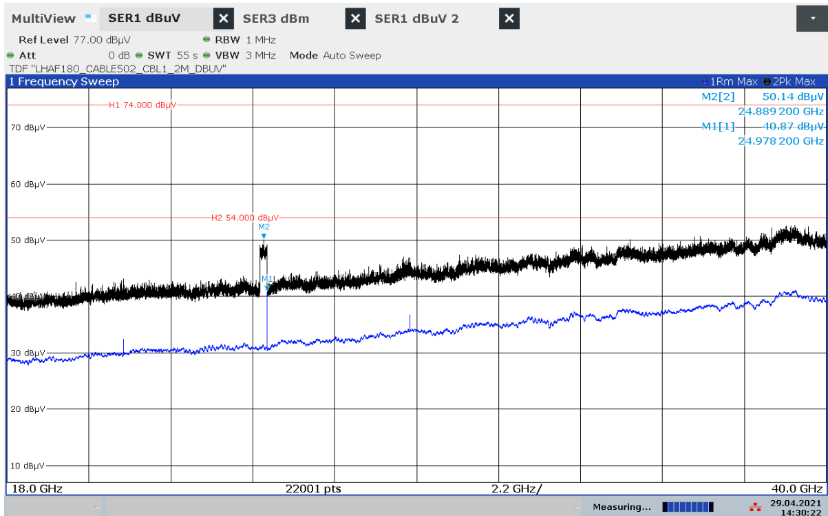
Plot 17: 18 GHz – 40 GHz, normal mode
