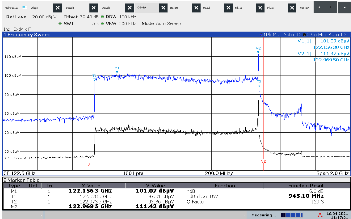
Plot 42: T_{nom} / V_{min}
