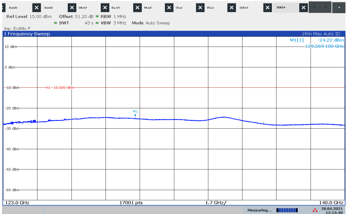
Plot 32: 123 GHz – 140 GHz, stopped mode (sweep stopped in the middle of the range of operation)
