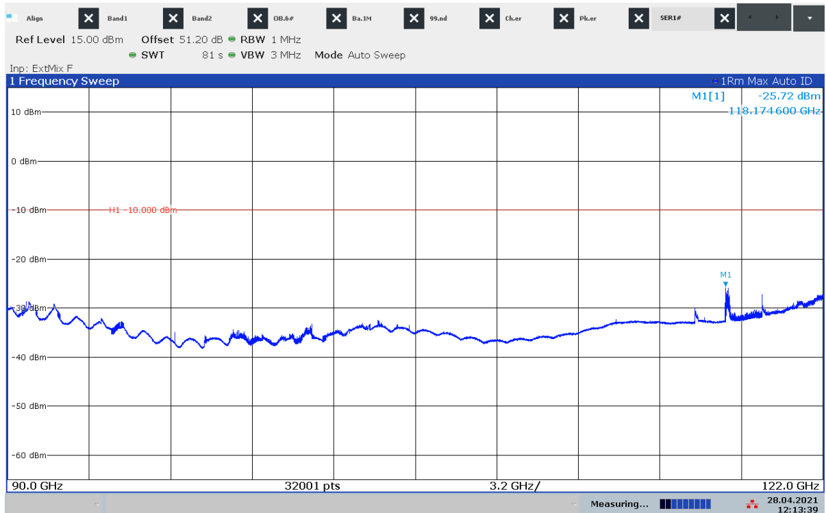
Plot 26: 90 GHz – 122 GHz, stopped mode (sweep stopped in the middle of the range of operation)
