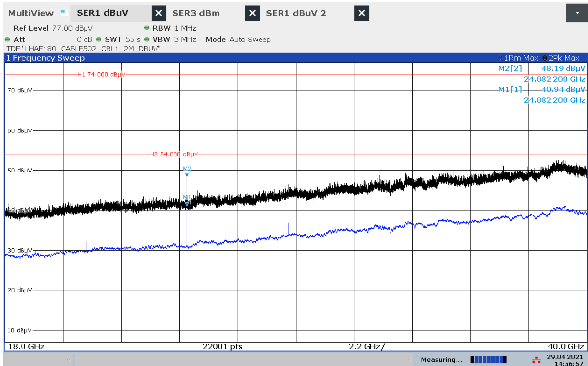
Plot 18: 18 GHz – 40 GHz, stopped mode (sweep stopped in the middle of the range of operation)
