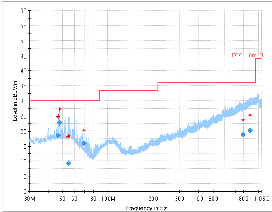
Plot 11: 30 MHz – 1 GHz, normal mode
