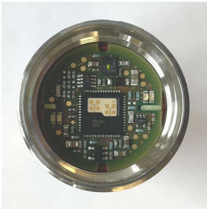
Back-Print and Front-Print inside housing
