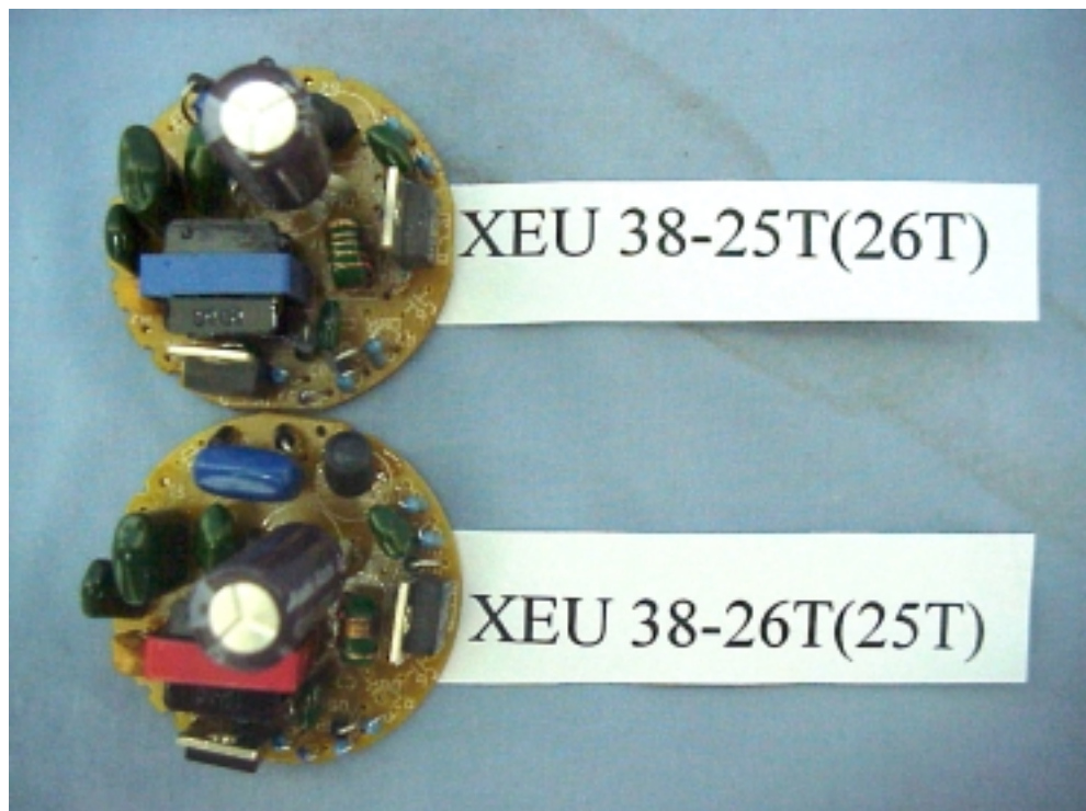
Figure 2 ENERGY SAVING LAMP (M/N: XEU38-T SERIAL) MAIN BOARD (COMPONENT SIDE)
