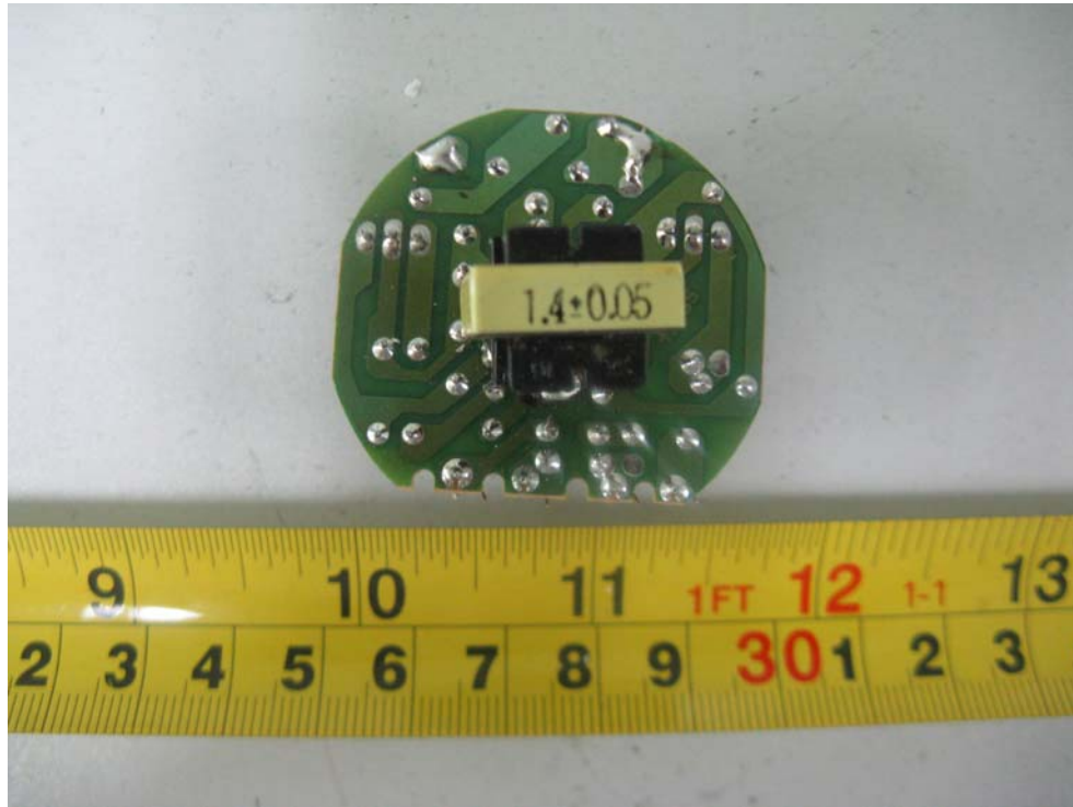
EUT – Main Board Bottom View (BU4-20D)
