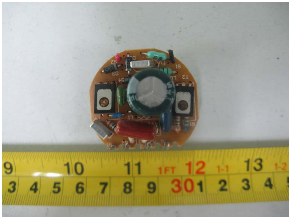
EUT – Main Board Top View (BU4-20D)
