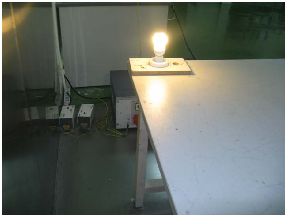
Conducted Emissions – Side View (BU4-14D)
