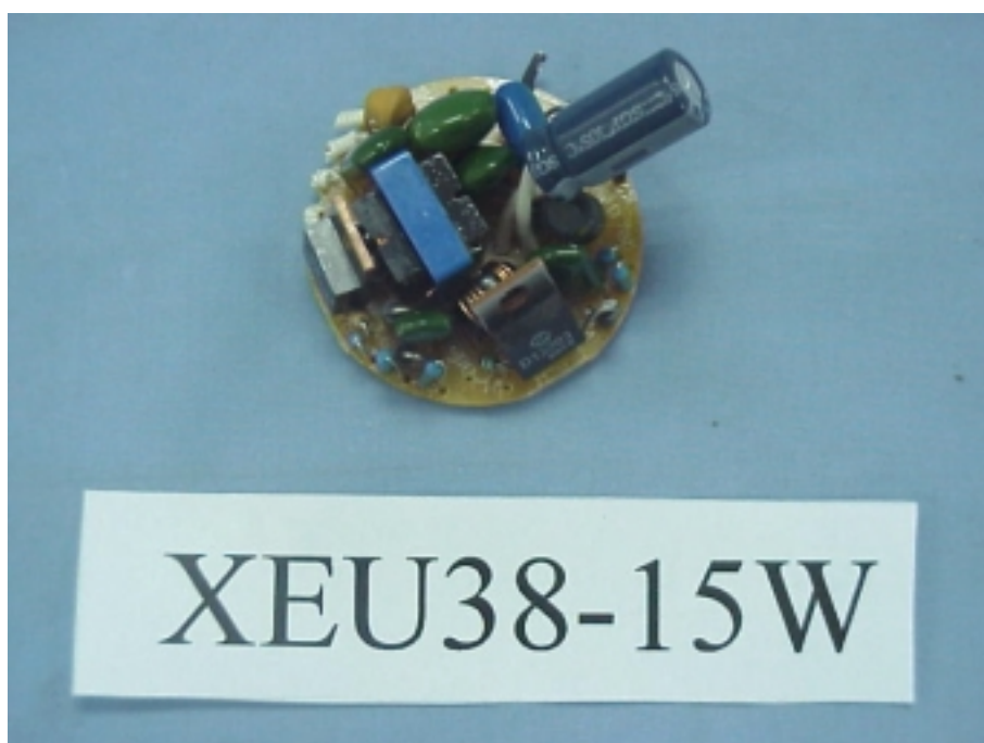
Figure 2 Energy Saving Lamp (M/N: XEU38-15W) MAIN BOARD (COMPONENT SIDE)
