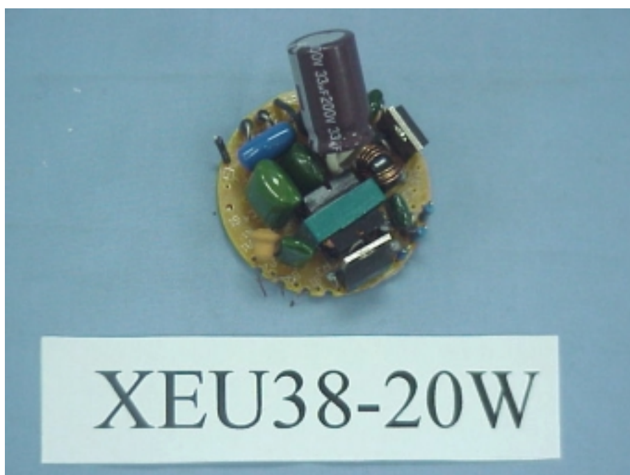
Figure 8 Energy Saving Lamp (M/N: XEU38-20W) MAIN BOARD (COMPONENT SIDE)
