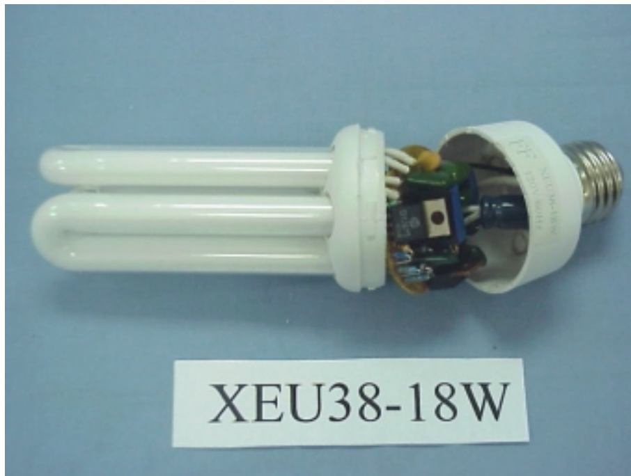
Figure 4 Energy Saving Lamp (M/N: XEU38-18W) COVER REMOVED
