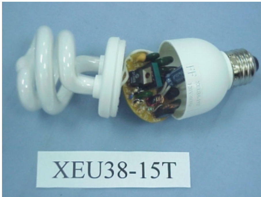
Figure 13 Energy Saving Lamp (M/N: XEU38-15T) COVER REMOVED
