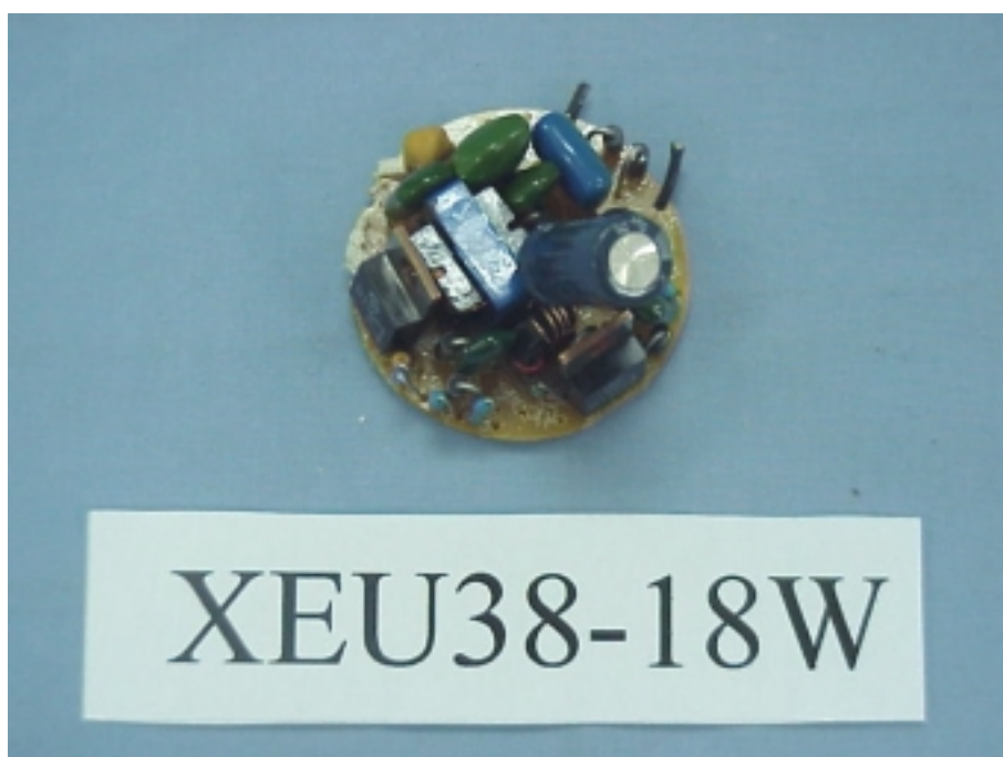
Figure 5 Energy Saving Lamp (M/N: XEU38-18W) MAIN BOARD (COMPONENT SIDE)
