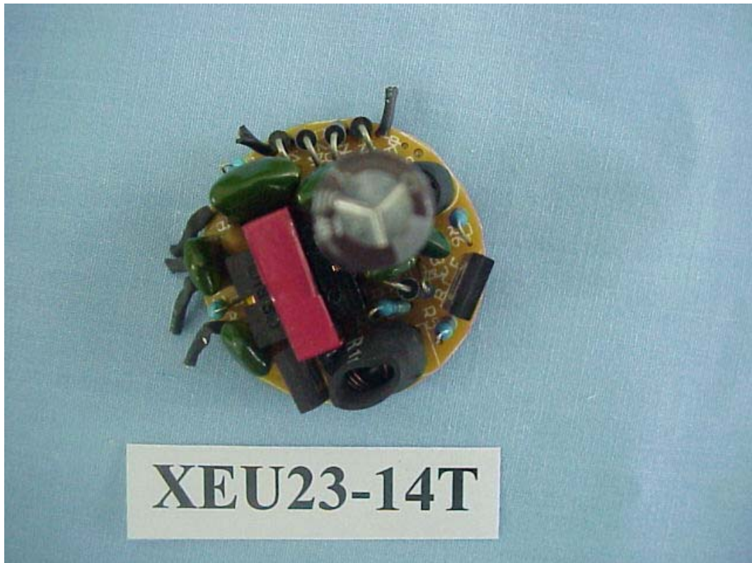
FIGURE 8 ELECTRONIC ENERGY SAVING LAMP (M/N: XEU23-14T) MAIN BOARD (COMPONENT SIDE)
