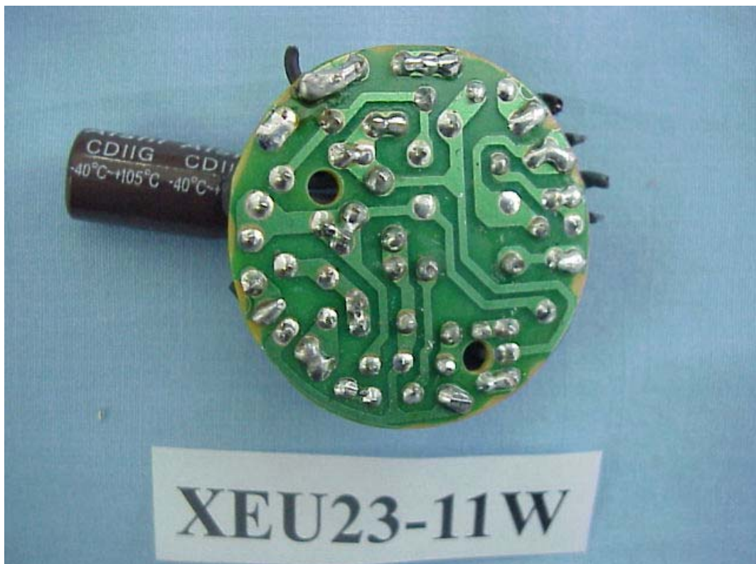
FIGURE 15 ELECTRONIC ENERGY SAVING LAMP (M/N: XEU23-11W) MAIN BOARD (SOLDERED SIDE)
