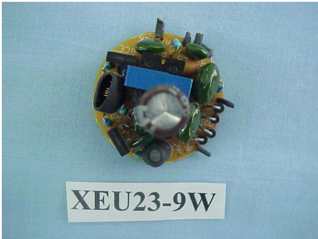
FIGURE 11 ELECTRONIC ENERGY SAVING LAMP (M/N: XEU23-9W) MAIN BOARD (COMPONENT SIDE)
