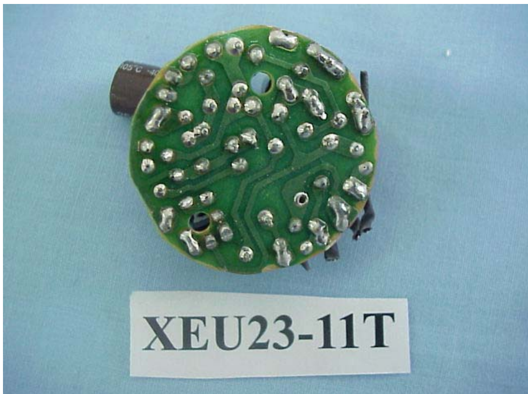
FIGURE 6 ELECTRONIC ENERGY SAVING LAMP (M/N: XEU23-11T) MAIN BOARD (SOLDERED SIDE)
