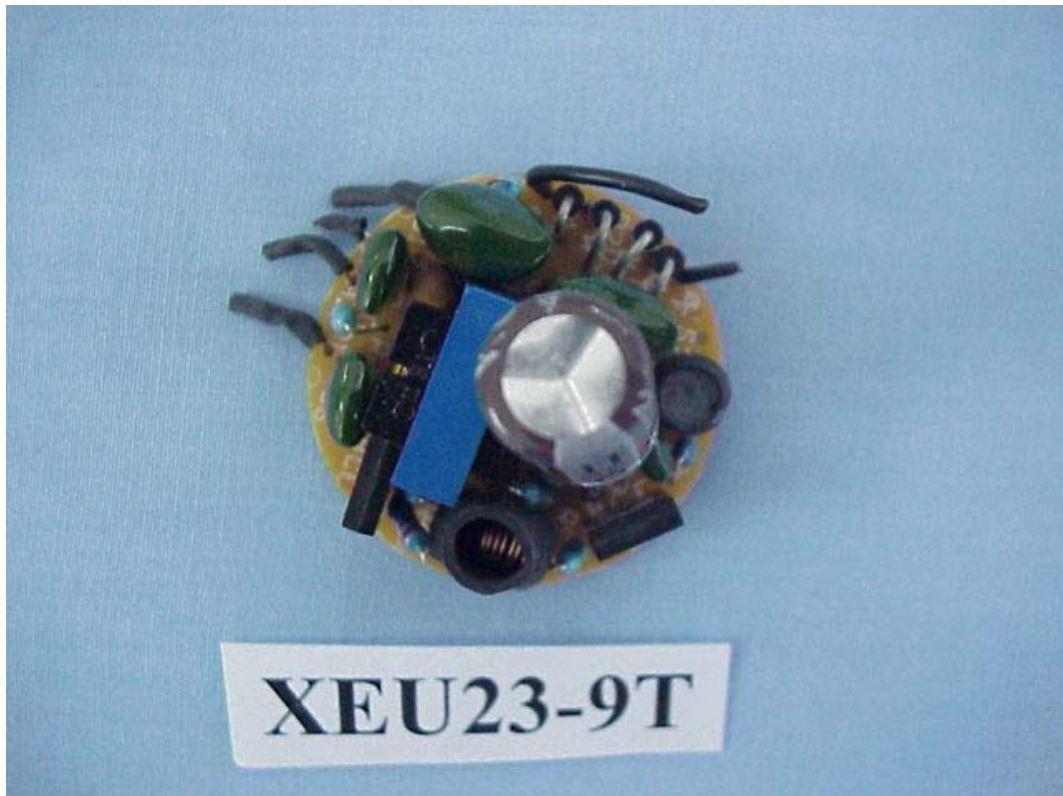
FIGURE 2 ELECTRONIC ENERGY SAVING LAMP (M/N: XEU23-9T) MAIN BOARD (COMPONENT SIDE)
