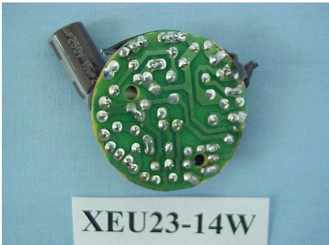
FIGURE 18 ELECTRONIC ENERGY SAVING LAMP (M/N: XEU23-14W) MAIN BOARD (SOLDERED SIDE)
