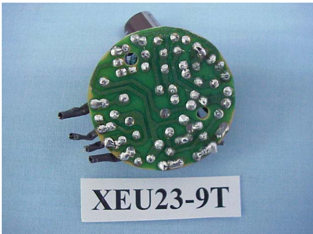
FIGURE 3 ELECTRONIC ENERGY SAVING LAMP (M/N: XEU23-9T) MAIN BOARD (SOLDERED SIDE)
