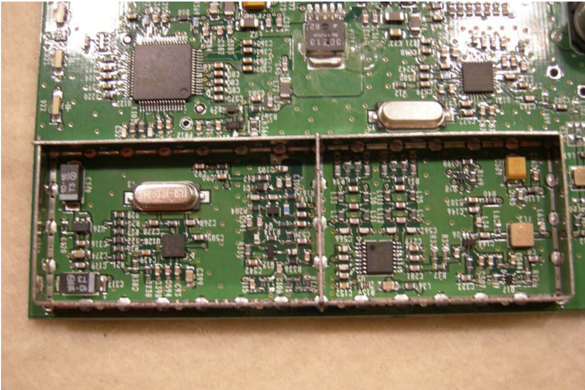
Figure A5: Main Board – Top without RF Shield
