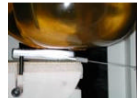
Fig. 18 Head SAR Test Setup
