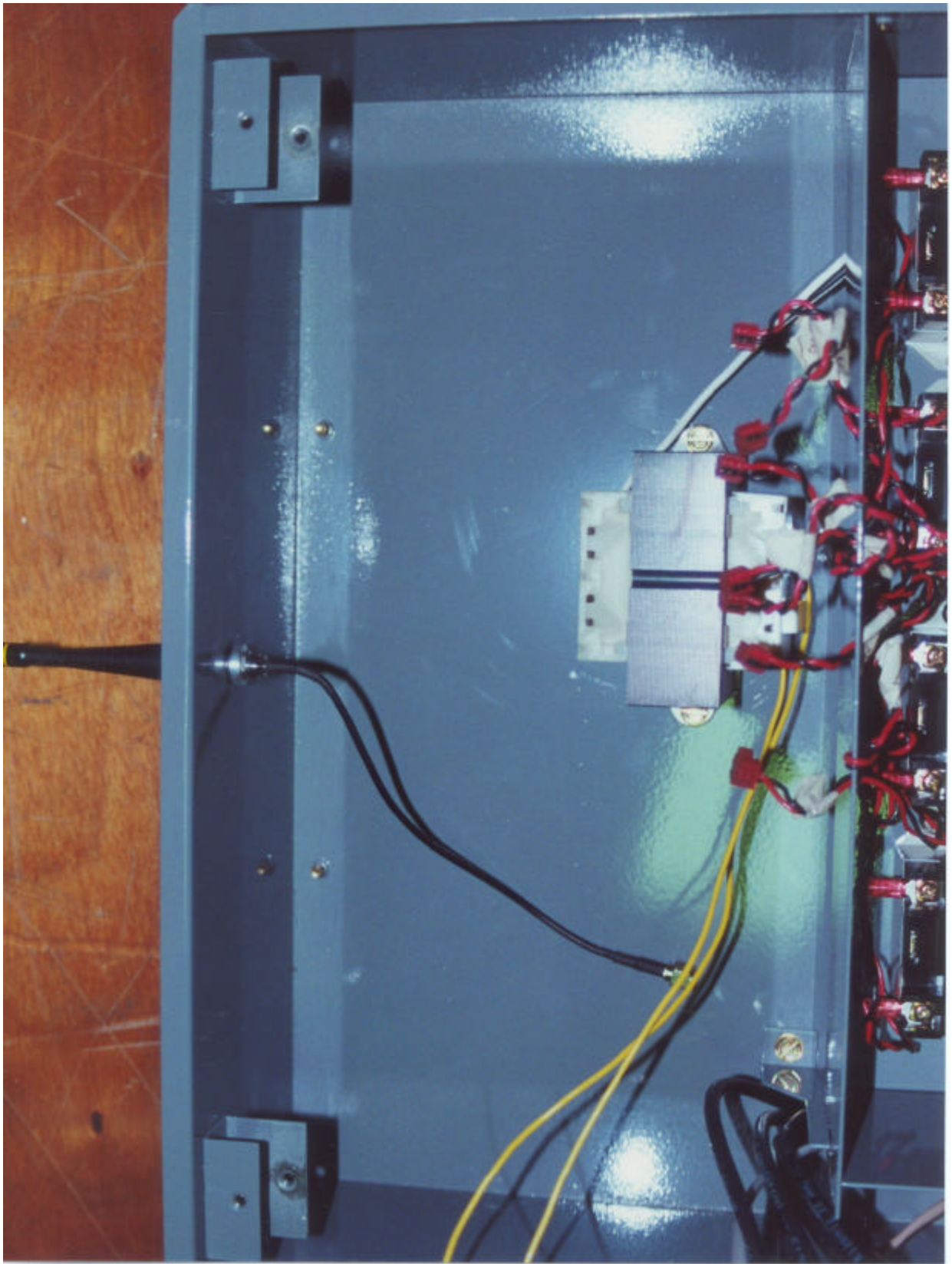
INSIDE VIEW OF COMMAND CENTER (TRANSFORMER/ANTENNA)
