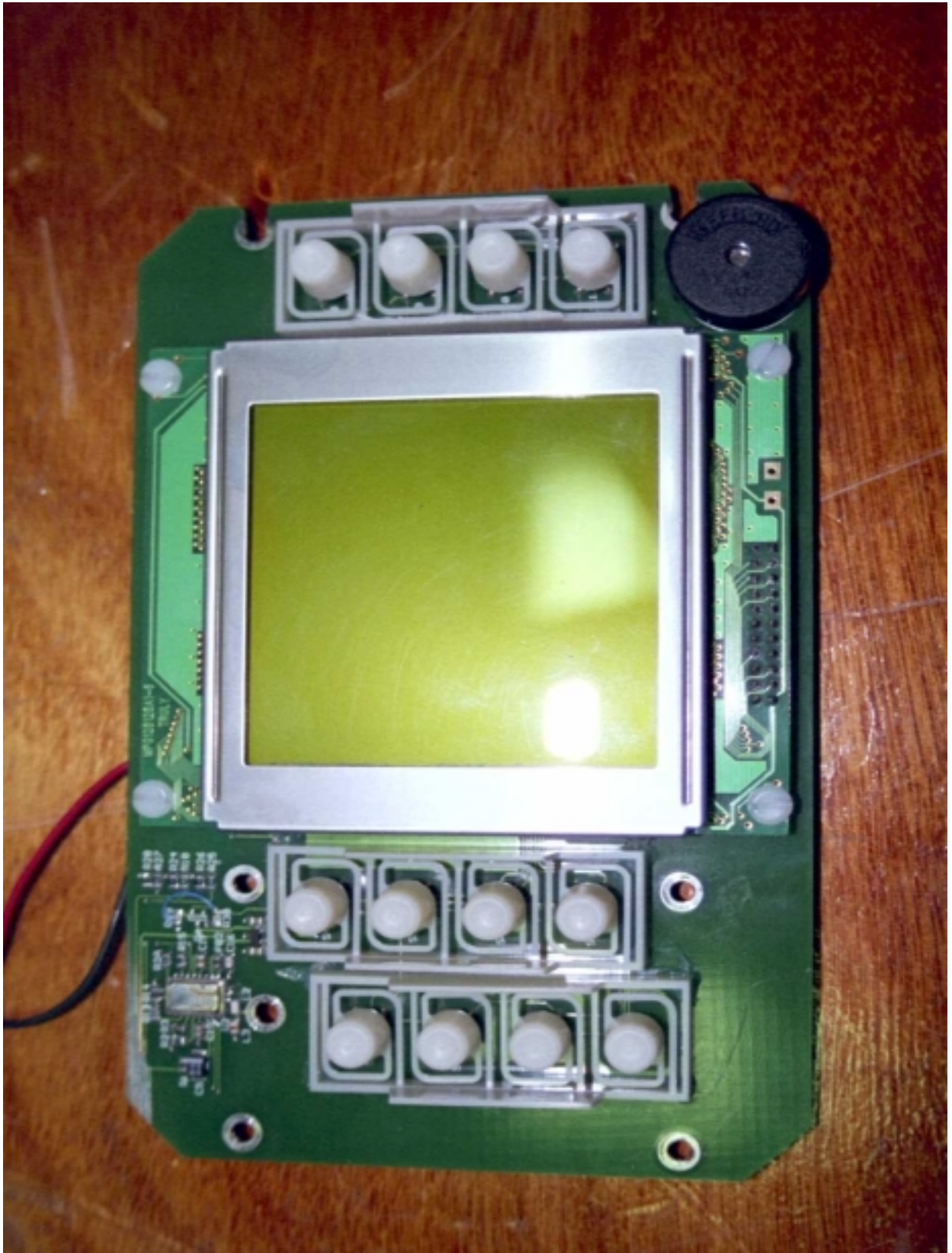
TOP VIEW OF REMOTE CONTROL CIRCUIT BOARD
