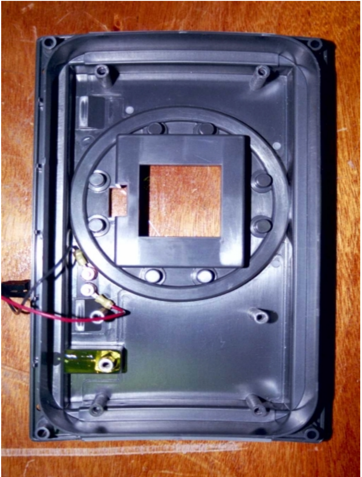
INSIDE VIEW OF REMOTE CONTROL BOTTOM COVER
