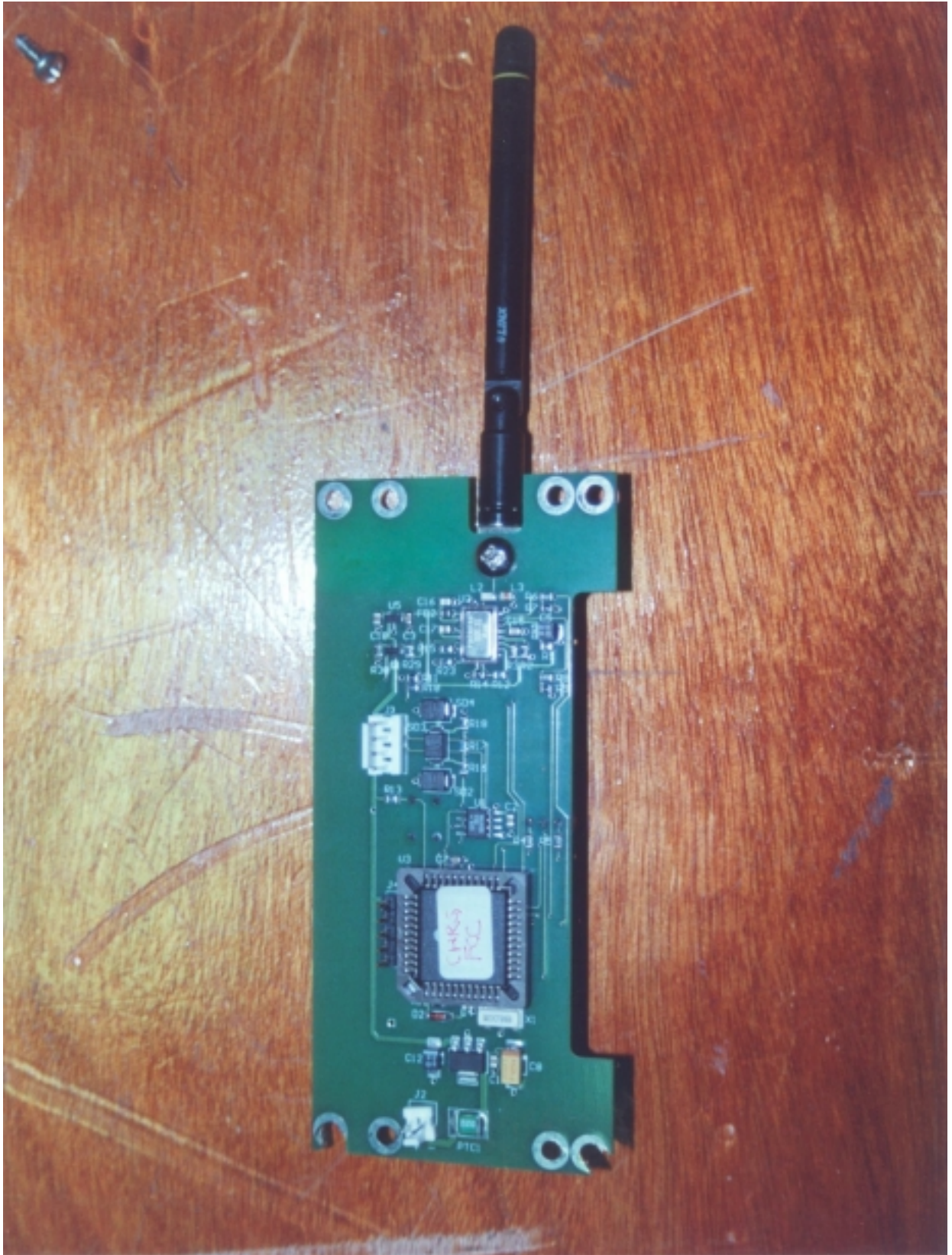
TOP VIEW OF BATTERY CHARGER CIRCUIT BOARD
