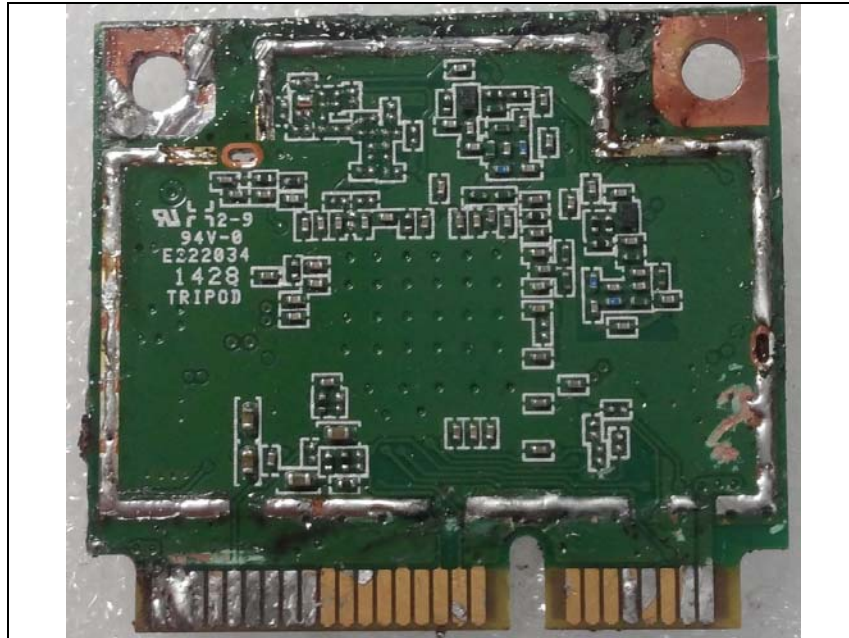
RF Module(Shields removed_Bottom)
