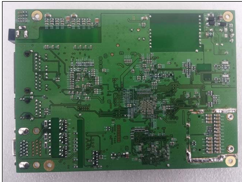
Main board (Bottom)
