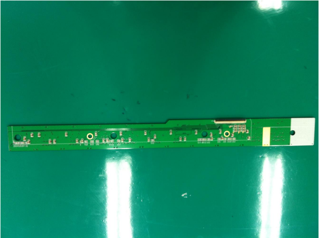
Gate Board_overall_back
