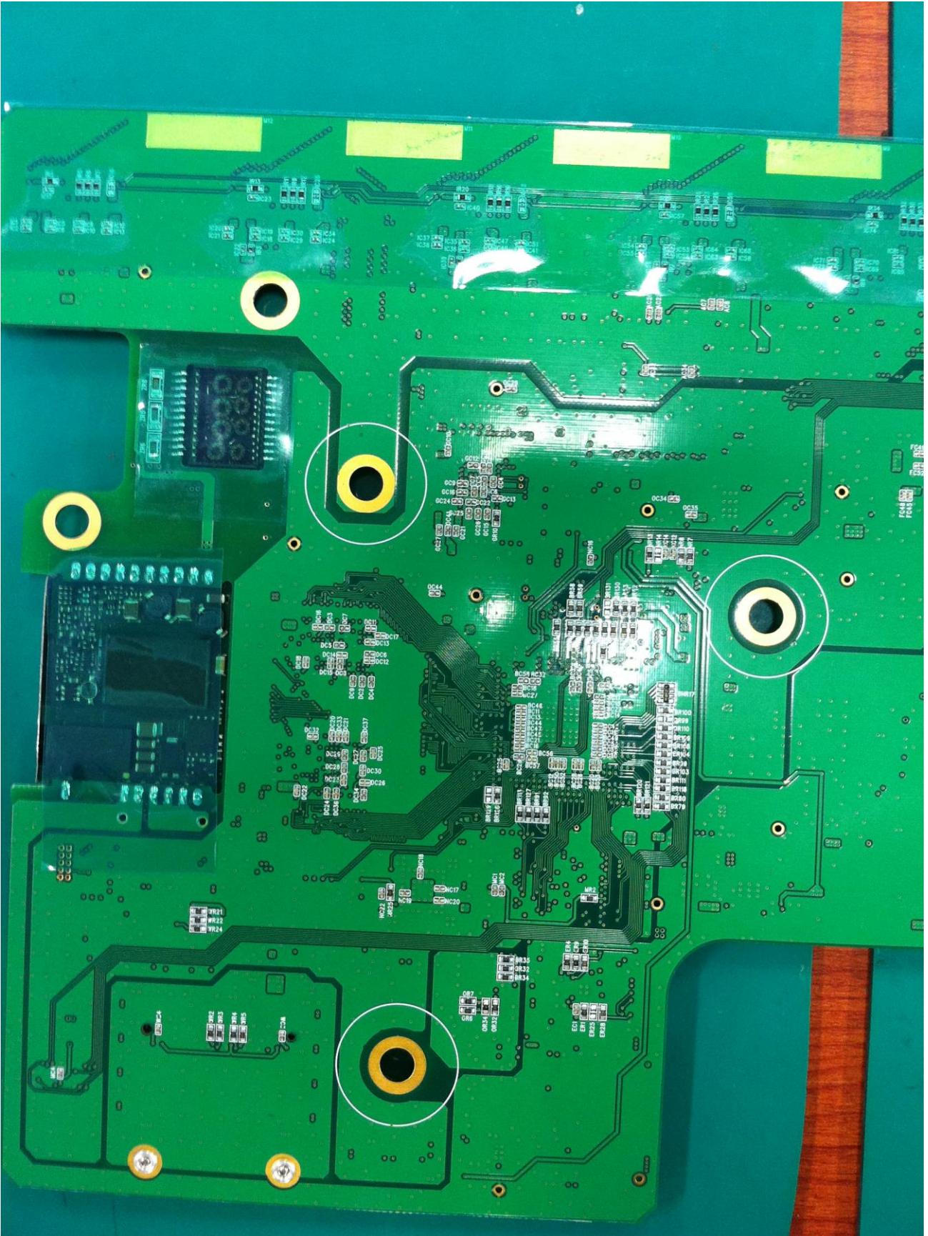
Main board_back_1
