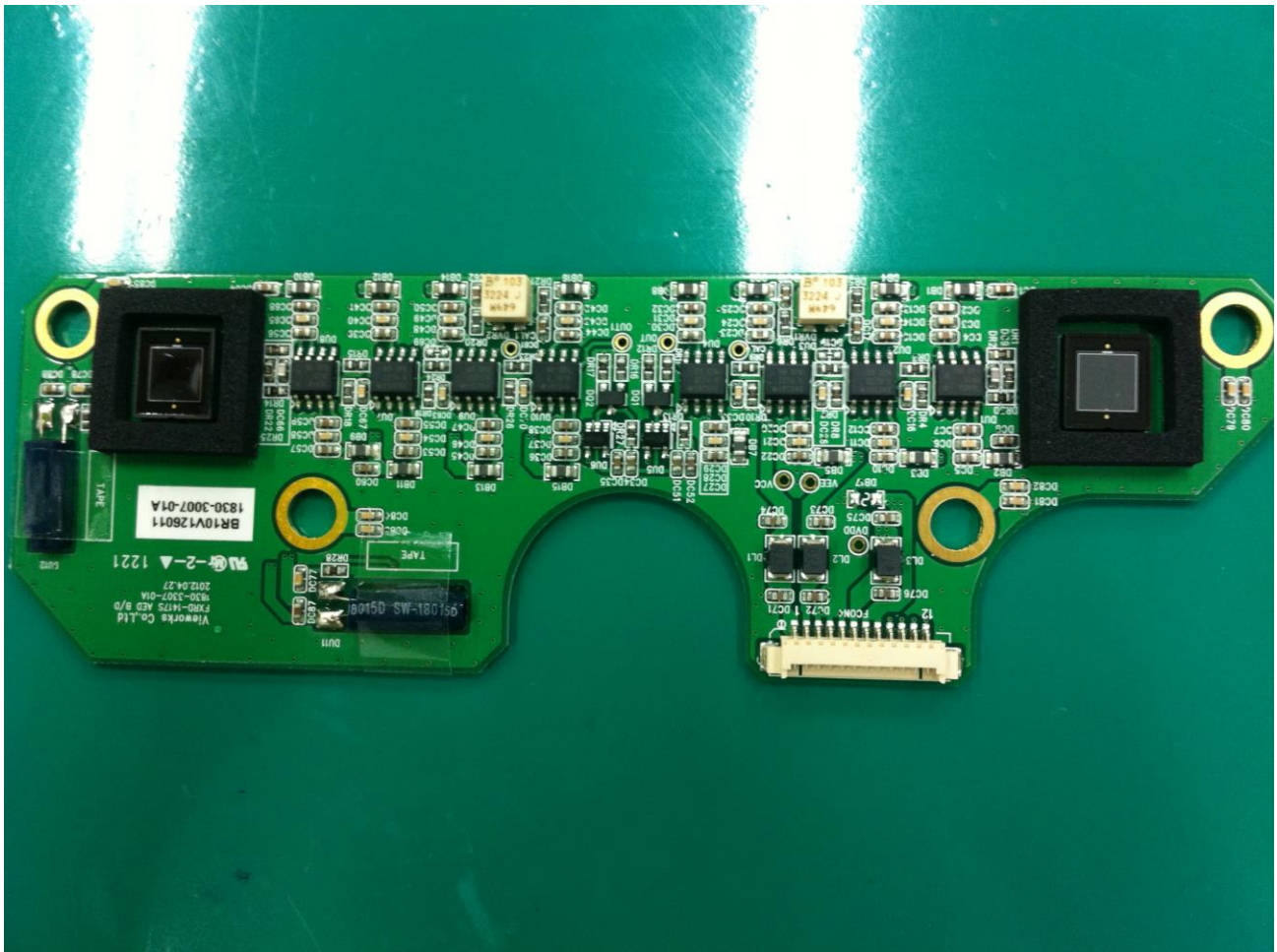
AED Board_front
