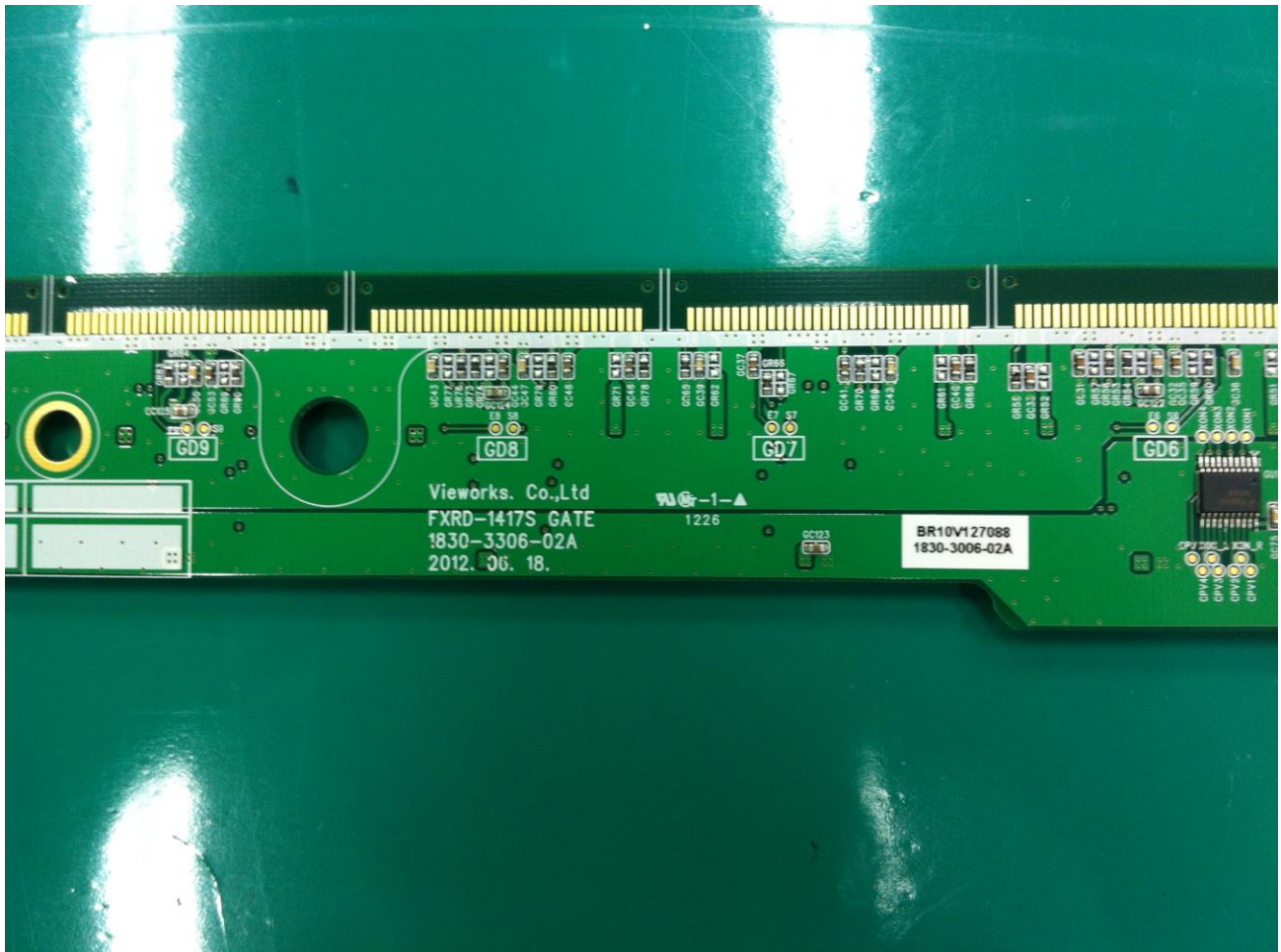
Gate Board_front_1
